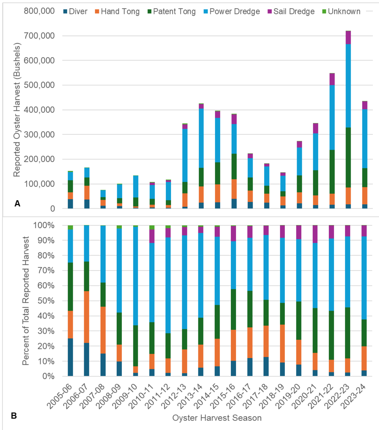
Figure 9. Annual oyster harvest by gear from the Maryland portion of Chesapeake Bay a) in bushels, b) as a percentage of the annual harvest during the 2005-2006 to 2023-2024 harvest seasons.
