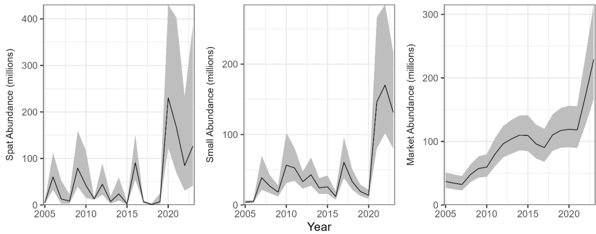
Figure 94. Estimated abundance of spat, small, and markets oysters during 2005-2023 in Mid Choptank River. The lines indicate the estimated abundances, and the shaded areas indicate approximate 95% confidence intervals.
