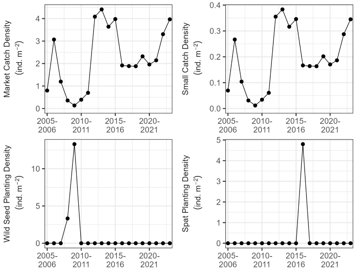
Figure 105. Catch density of market oysters, catch density of small oysters, wild seed planting density, and spat planting density during 2005-2023 in Broad Creek. Density was calculated as the number of individuals divided by habitat area for each data source.
