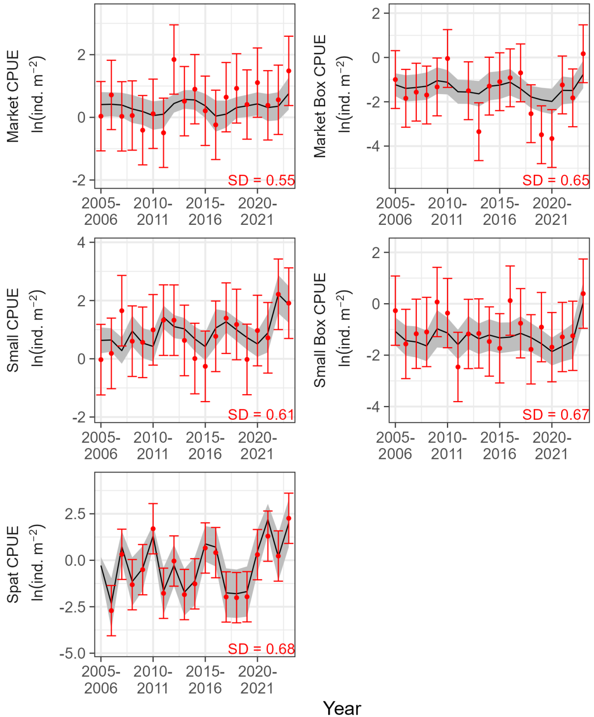
Figure 24. Estimated (line) and observed (points) values for Smith Creek. Variable and symbol definitions are the same as Figure 12.
