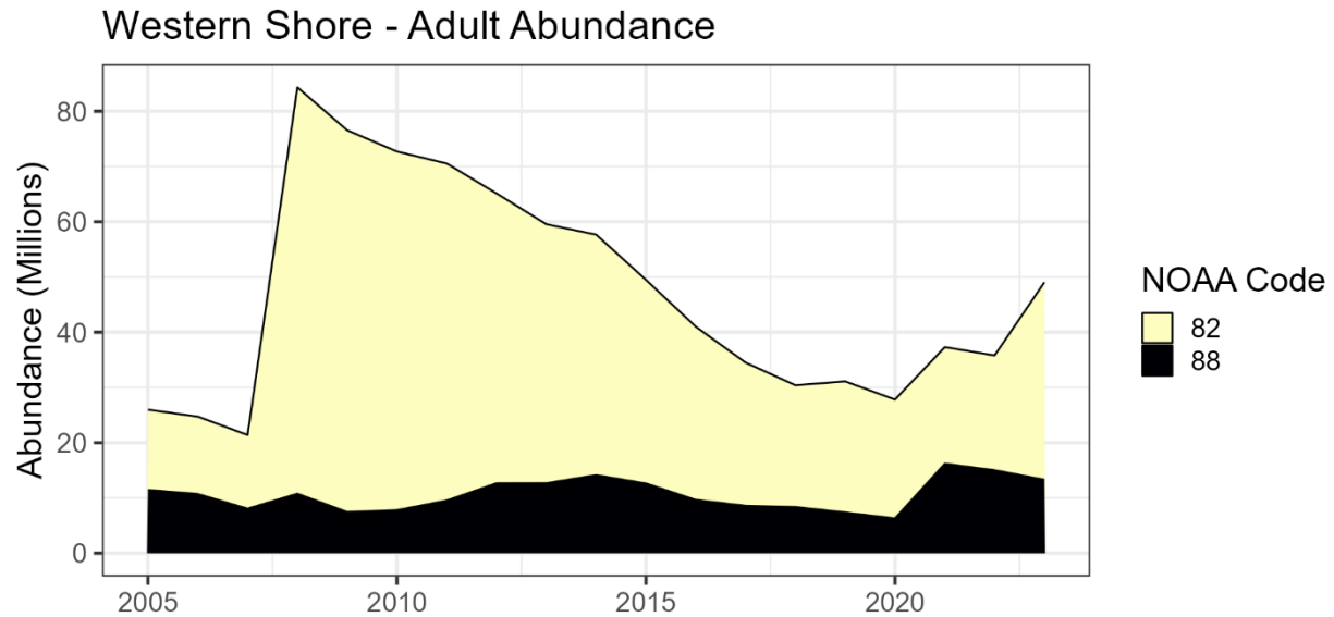
Figure 187. Estimated adult oyster abundance among modeled NOAA codes in the Western Shore Region under Maryland management during 2005-2023.
