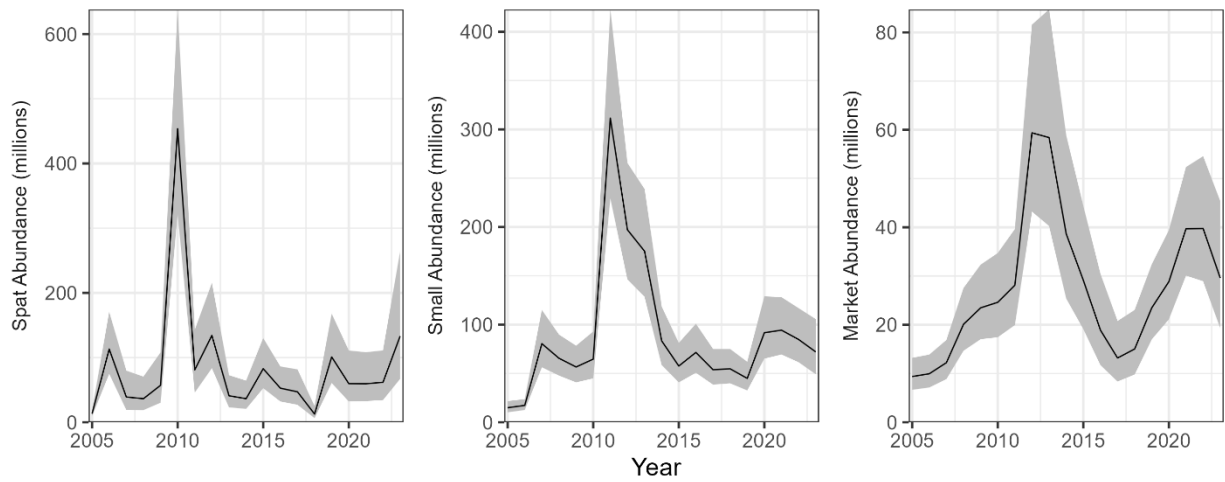
Figure 72. Estimated abundance of spat, small, and markets oysters during 2005-2023 in Pocomoke Sound. The lines indicate the estimated abundances, and the shaded areas indicate approximate 95% confidence intervals.
