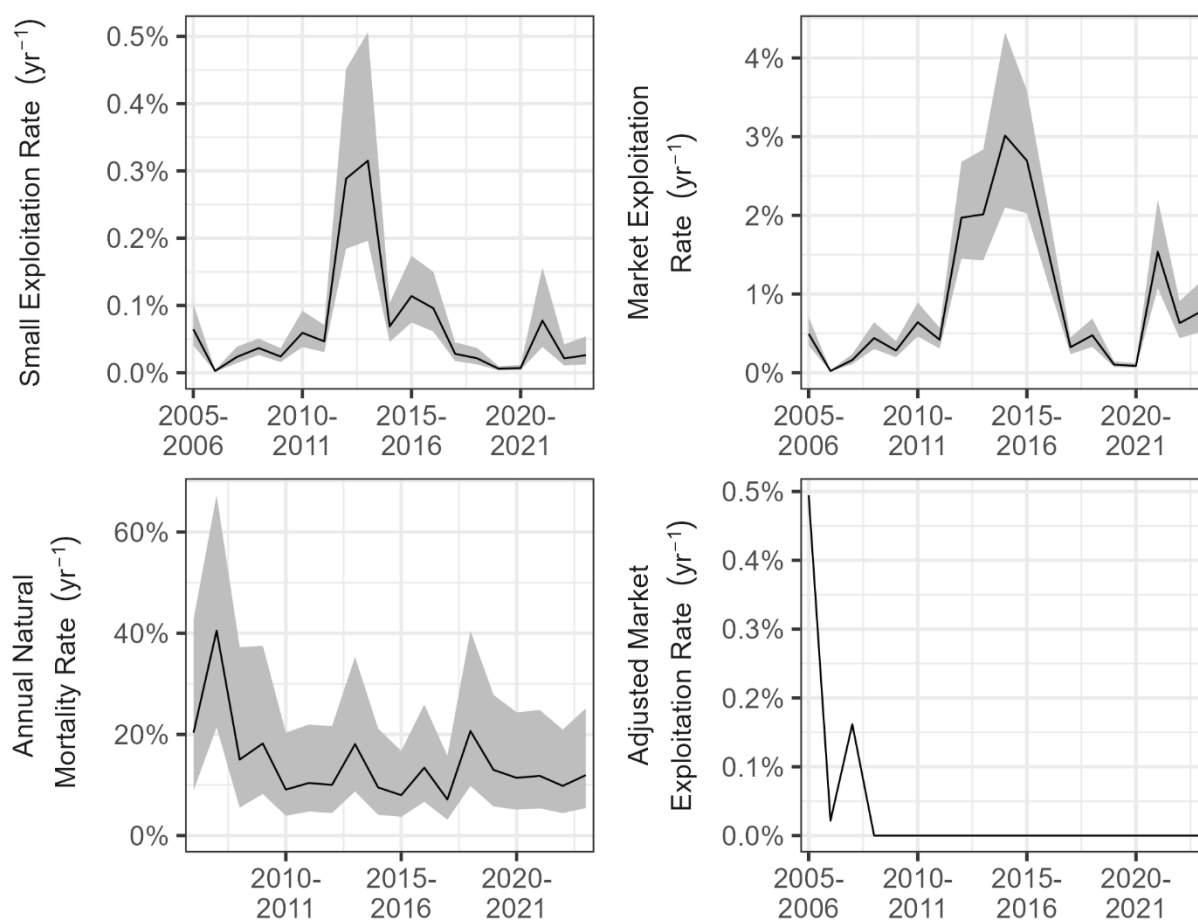
Figure 149. Estimated small exploitation rate, market exploitation rate, annual natural mortality rate, and adjusted market exploitation rate during 2005-2023 in Wicomico River (West). The shaded areas indicate approximate 95% confidence intervals.
