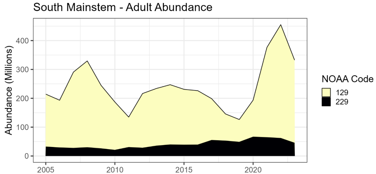
Figure 164. Estimated adult oyster abundance among modeled NOAA codes in the South Mainstem Region under Maryland management during 2005-2023.
