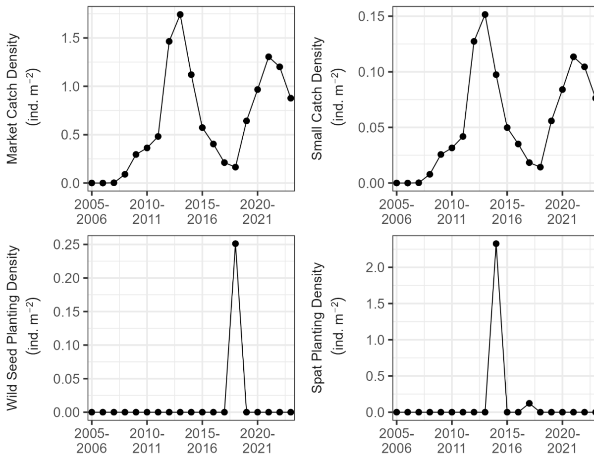
Figure 62. Catch density of market oysters, catch density of small oysters, wild seed planting density, and spat planting density during 2005-2023 in Fishing Bay. Density was calculated as the number of individuals divided by habitat area for each data source.
