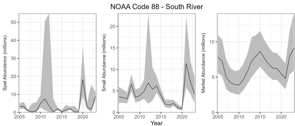
Figure 194. Estimated abundance of spat, small, and markets oysters during 2005-2023 in South River. The lines indicate the estimated abundances, and the shaded areas indicate approximate 95% confidence intervals.
