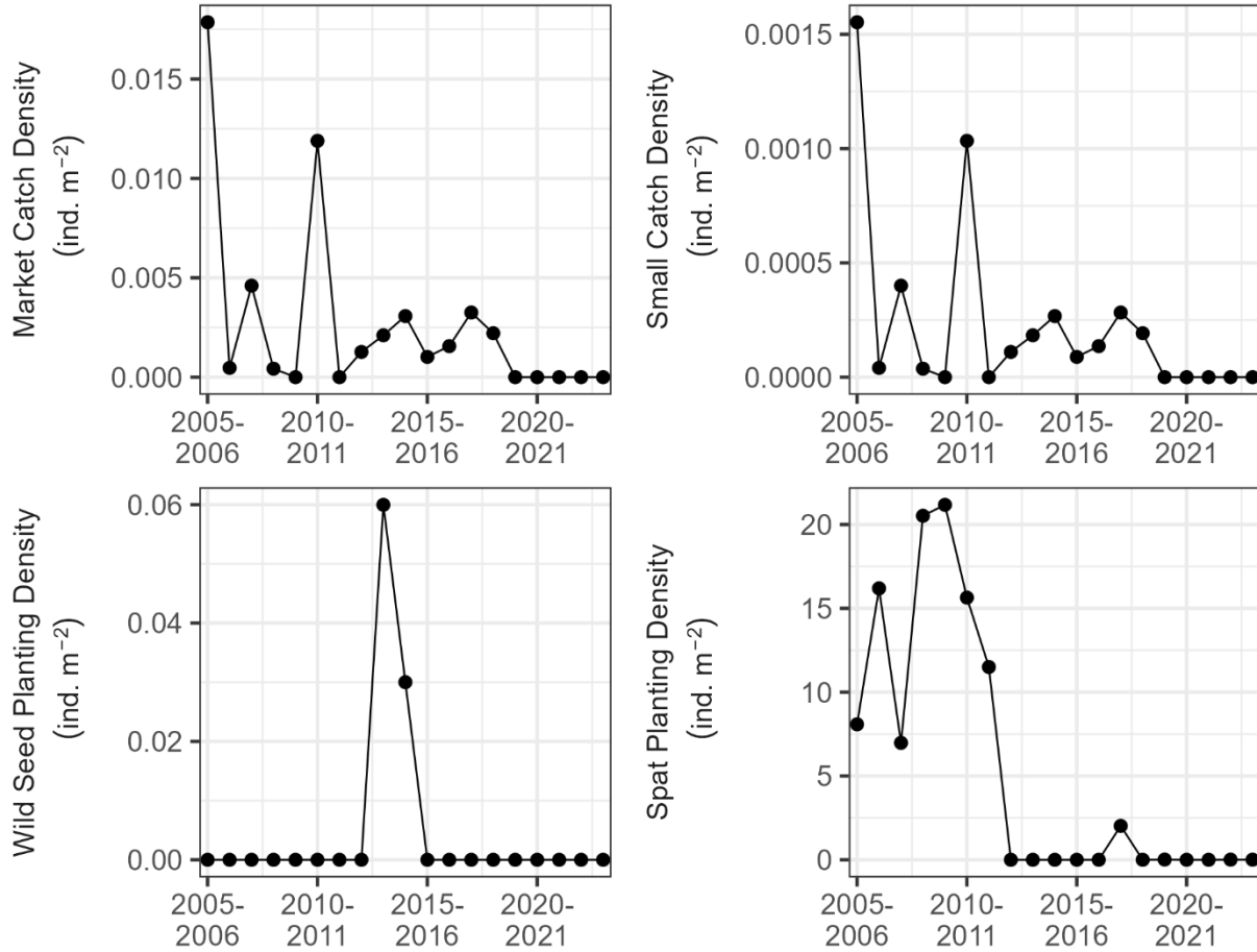
Figure 99. Catch density of market oysters, catch density of small oysters, wild seed planting density, and spat planting density during 2005-2023 in Upper Choptank River. Density was calculated as the number of individuals divided by habitat area for each data source.
