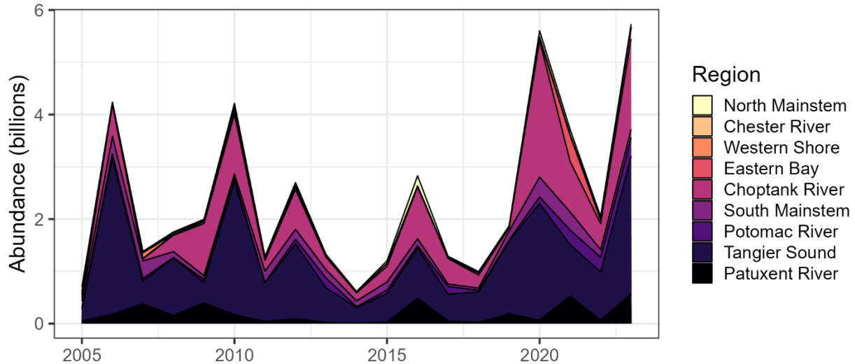
All modeled NOAA Codes by Region - Spat Abundance
