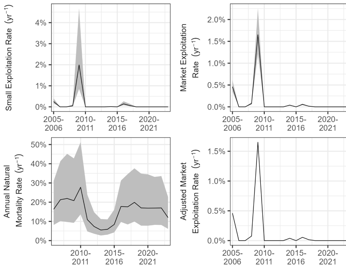
Figure 133. Estimated small exploitation rate, market exploitation rate, annual natural mortality rate, and adjusted market exploitation rate during 2005-2023 in Wye River. The shaded areas indicate approximate 95% confidence intervals.
