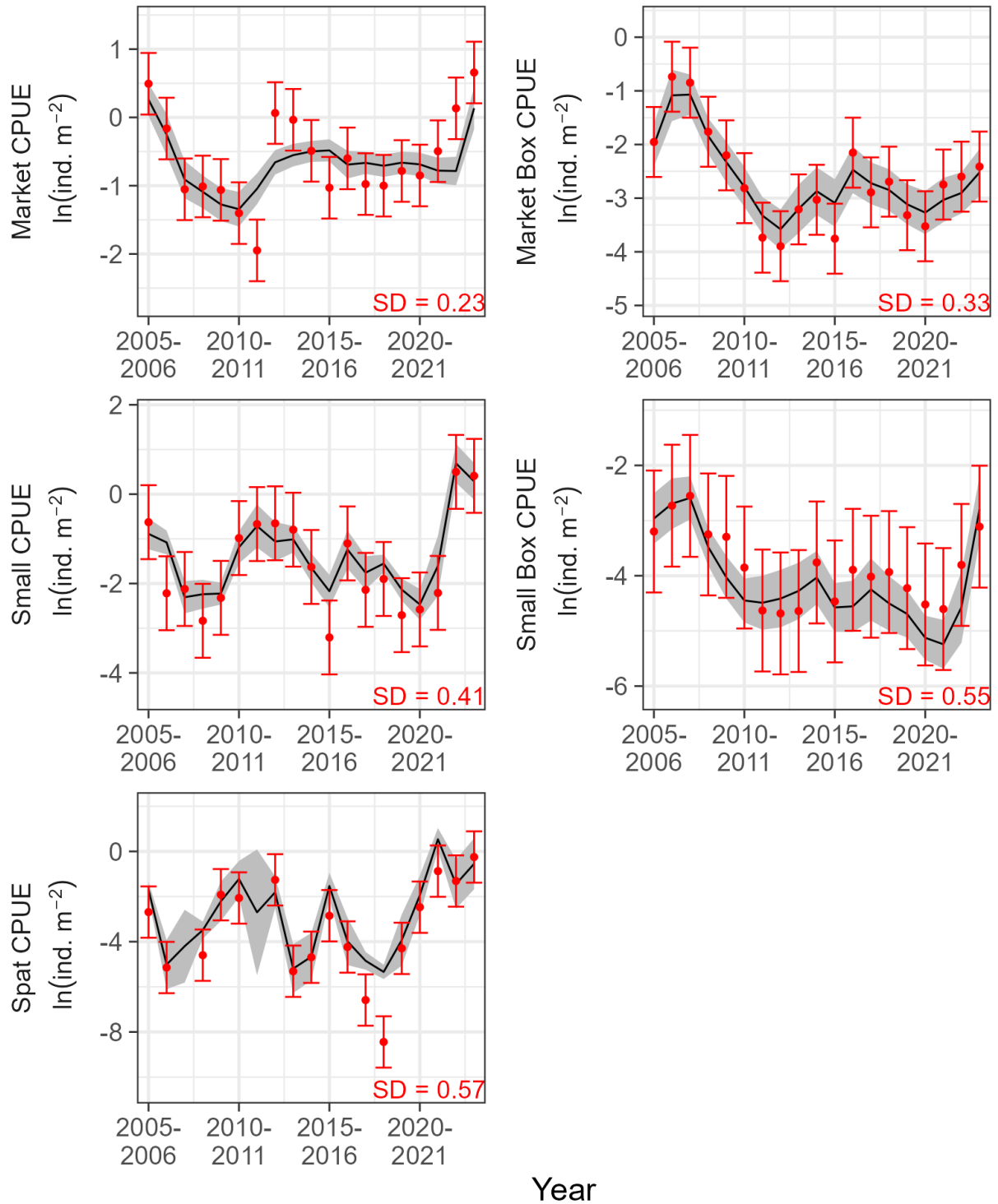
Figure 14. Estimated (line) and observed (points) values for Eastern Bay. Variable and symbol definitions are the same as Figure 12.
