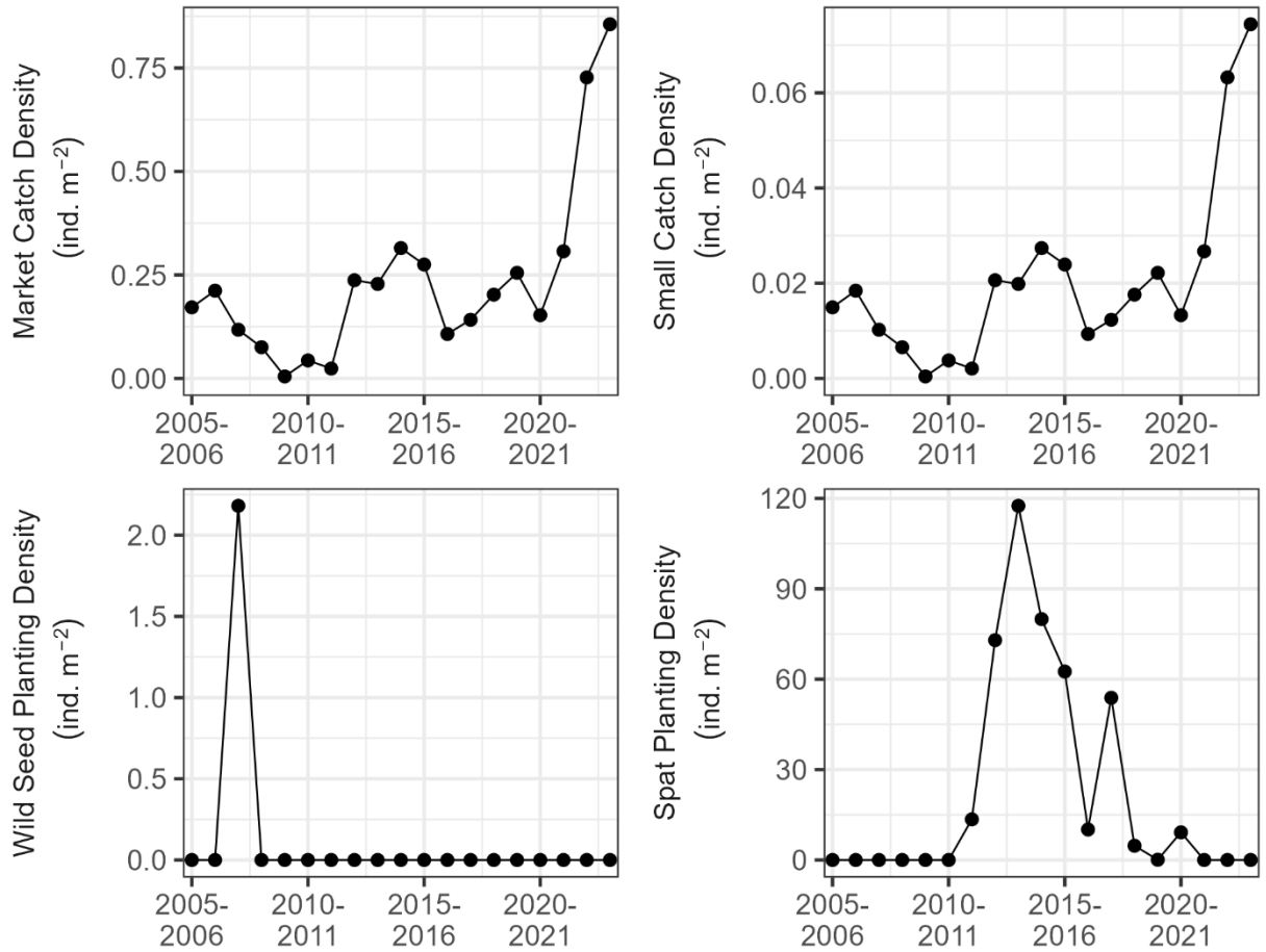
Figure 102. Catch density of market oysters, catch density of small oysters, wild seed planting density, and spat planting density during 2005-2023 in Harris Creek. Density was calculated as the number of individuals divided by habitat area for each data source.
