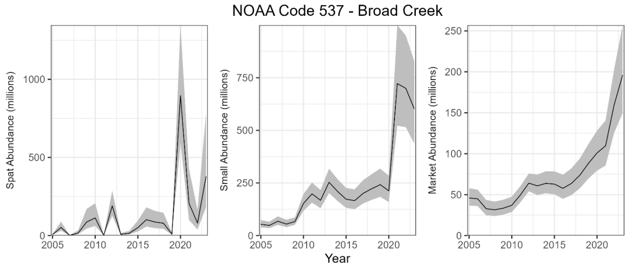
Figure 103. Estimated abundance of spat, small, and markets oysters during 2005-2023 in Broad Creek. The lines indicate the estimated abundances, and the shaded areas indicate approximate 95% confidence intervals.
