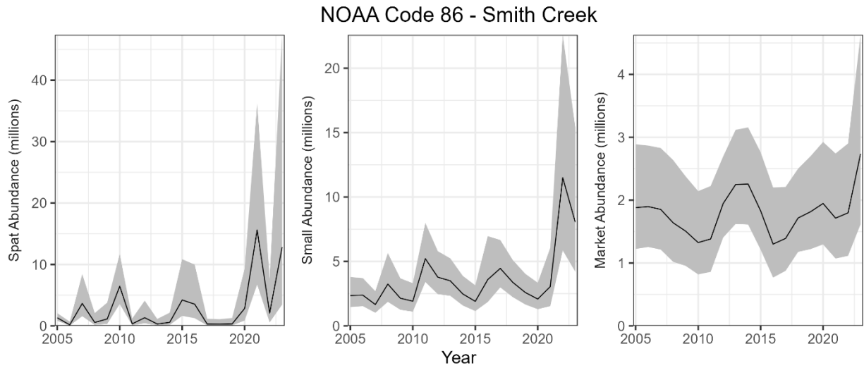
Figure 142. Estimated abundance of spat, small, and markets oysters during 2005-2023 in Smith Creek. The lines indicate the estimated abundances, and the shaded areas indicate approximate 95% confidence intervals.
