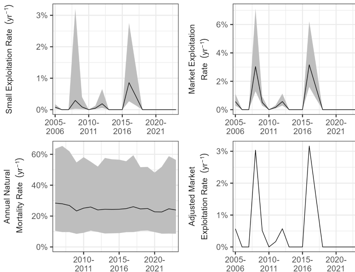
Figure 146. Estimated small exploitation rate, market exploitation rate, annual natural mortality rate, and adjusted market exploitation rate during 2005-2023 in Breton & St. Clements Bay. The shaded areas indicate approximate 95% confidence intervals.
