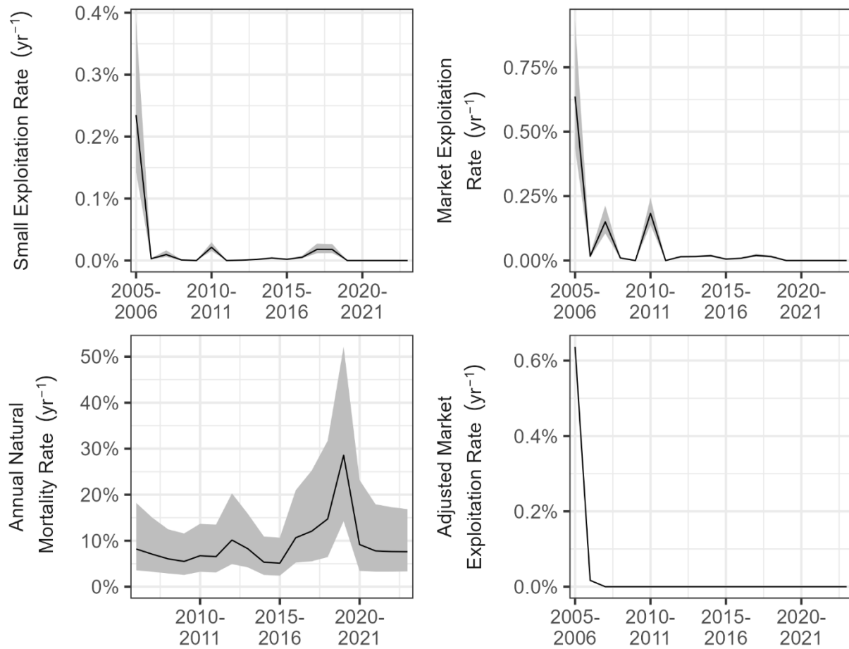
Figure 98. Estimated small exploitation rate, market exploitation rate, annual natural mortality rate, and adjusted market exploitation rate during 2005-2023 in Upper Choptank River. The shaded areas indicate approximate 95% confidence intervals.
