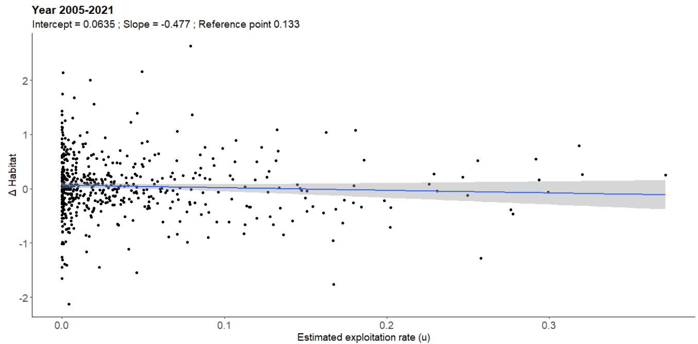
Figure 209 Results of sensitivity analysis for the exploitation rate reference point when using alternative ranges of years 2005-2021.
