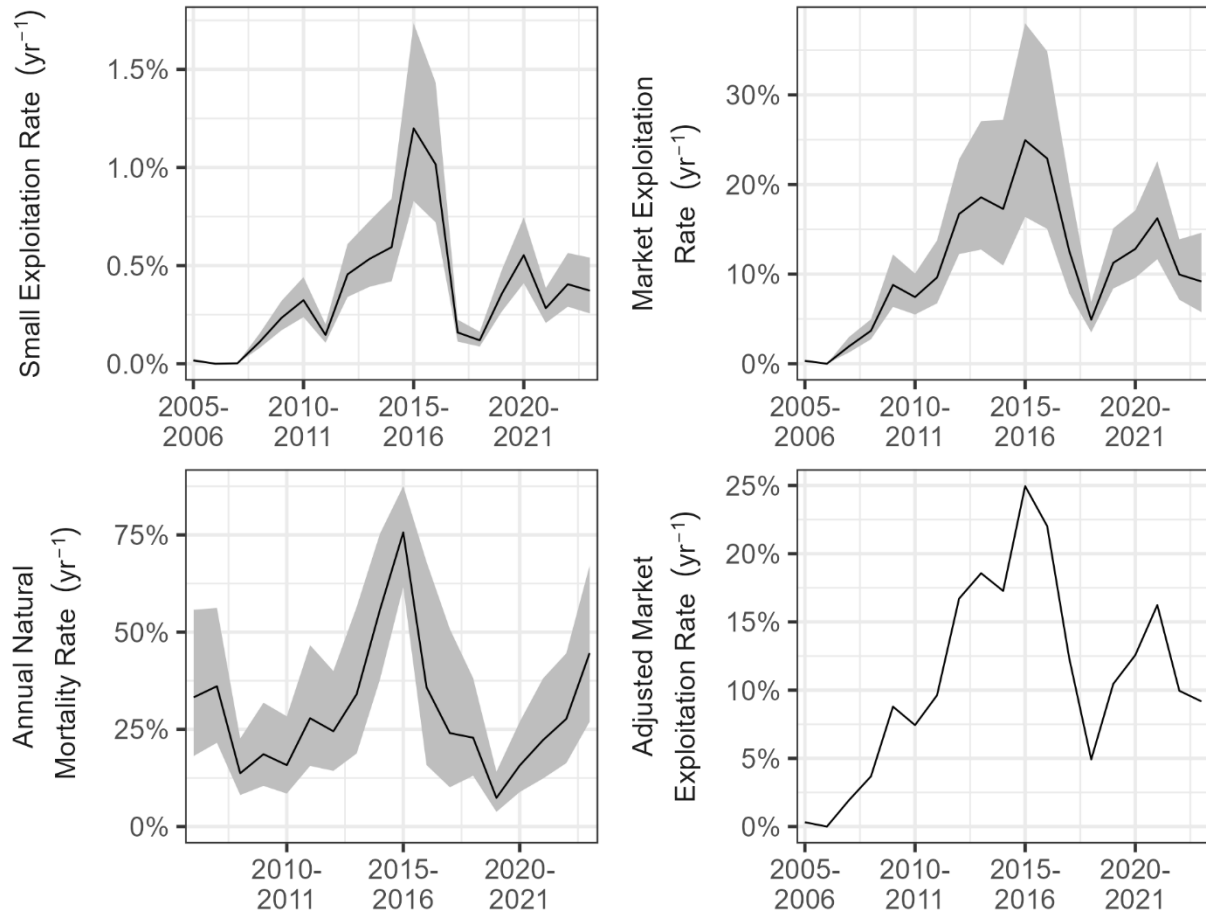
Figure 61. Estimated small exploitation rate, market exploitation rate, annual natural mortality rate, and adjusted market exploitation rate during 2005-2023 in Fishing Bay. The shaded areas indicate approximate 95% confidence intervals.
