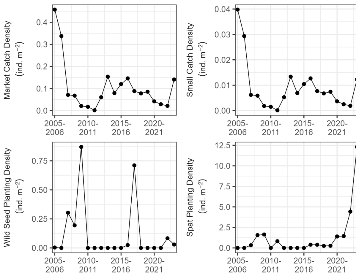
Figure 128. Catch density of market oysters, catch density of small oysters, wild seed planting density, and spat planting density during 2005-2023 in Eastern Bay. Density was calculated as the number of individuals divided by habitat area for each data source.
