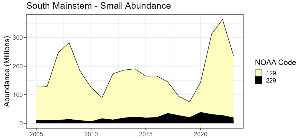
Figure 166. Estimated small oyster abundance among modeled NOAA codes in the South Mainstem Region under Maryland management during 2005-2023.
