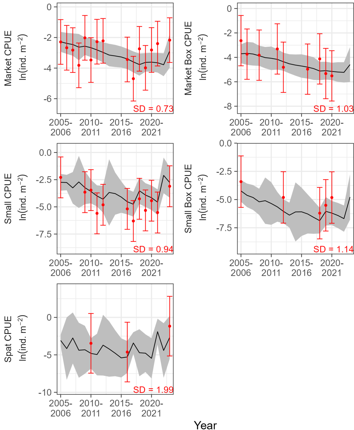
Figure 33. Estimated (line) and observed (points) values for Breton & St. Clement's Bay. Variable and symbol definitions are the same as Figure 12.
