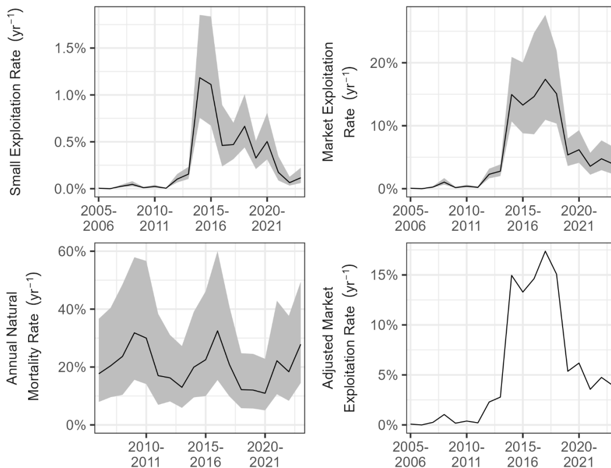
Figure 143. Estimated small exploitation rate, market exploitation rate, annual natural mortality rate, and adjusted market exploitation rate during 2005-2023 in Smith Creek. The shaded areas indicate approximate 95% confidence intervals.
