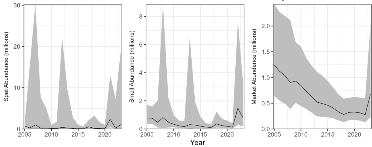
Figure 145. Estimated abundance of spat, small, and markets oysters during 2005-2023 in Breton & St. Clements Bay. The lines indicate the estimated abundances, and the shaded areas indicate approximate 95% confidence intervals.
