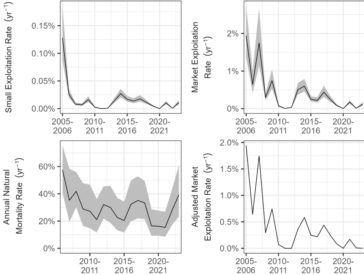
Figure 67. Estimated small exploitation rate, market exploitation rate, annual natural mortality rate, and adjusted market exploitation rate during 2005-2023 in Manokin River. The shaded areas indicate approximate 95% confidence intervals.
