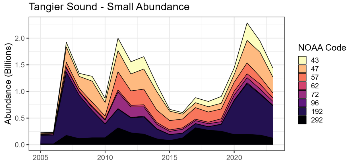
Figure 58. Estimated small oyster abundance among modeled NOAA codes in the Tangier Sound Region under Maryland management during 2005-2023.
