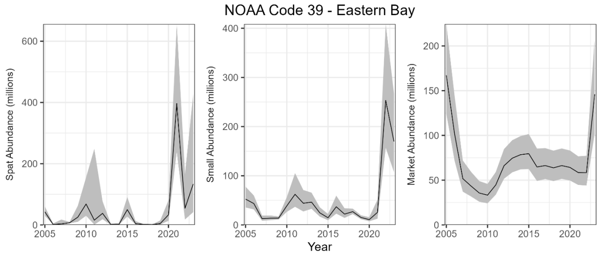
Figure 126. Estimated abundance of spat, small, and markets oysters during 2005-2023 in Eastern Bay. The lines indicate the estimated abundances, and the shaded areas indicate approximate 95% confidence intervals.
