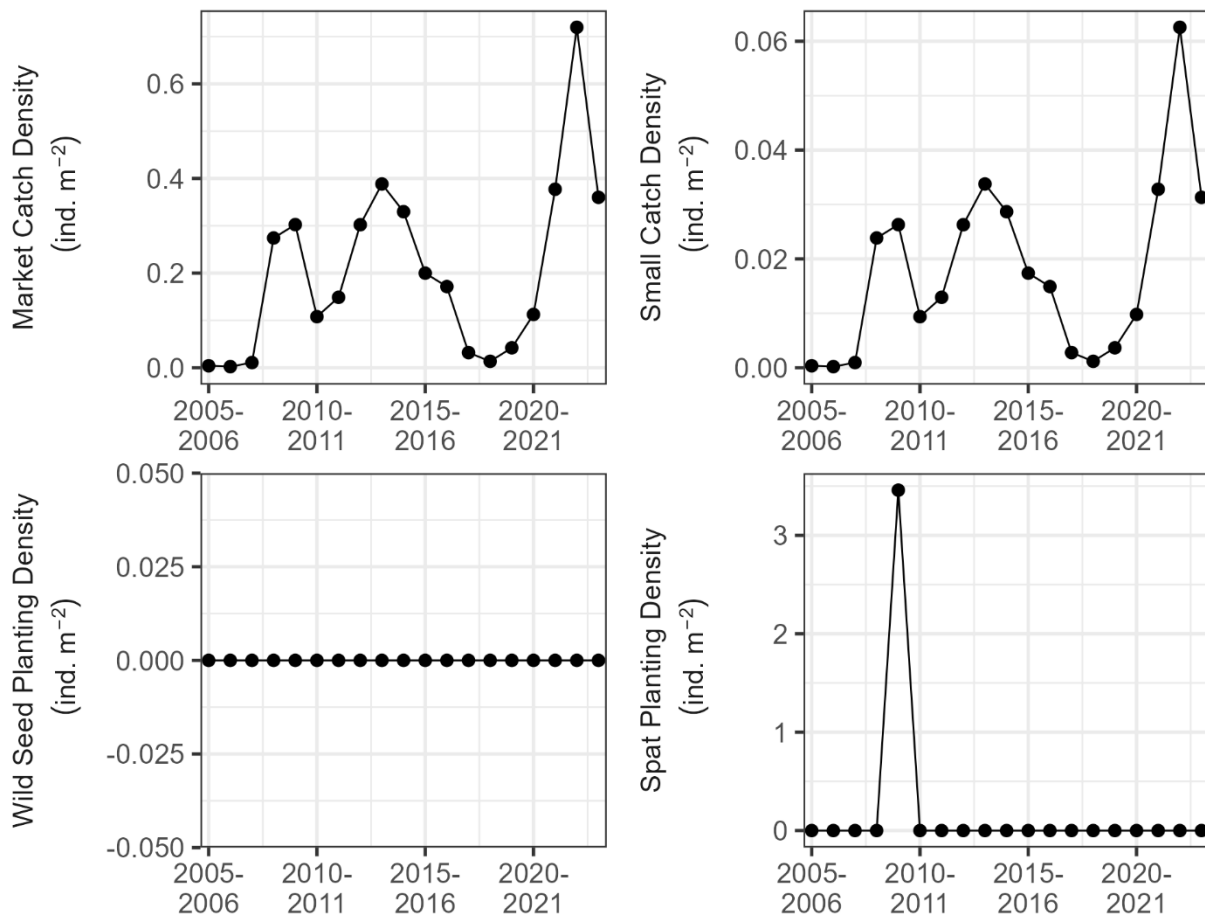
Figure 65. Catch density of market oysters, catch density of small oysters, wild seed planting density, and spat planting density during 2005-2023 in Honga River. Density was calculated as the number of individuals divided by habitat area for each data source.
