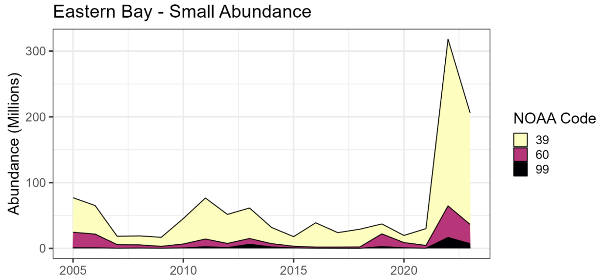
Figure 124. Estimated small oyster abundance among modeled NOAA codes in the Eastern Bay Region under Maryland management during 2005-2023.
