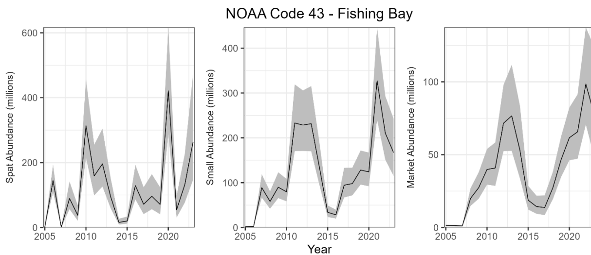
Figure 60. Estimated abundance of spat, small, and markets oysters during 2005-2023 in Fishing Bay. The lines indicate the estimated abundances, and the shaded areas indicate approximate 95% confidence intervals.
