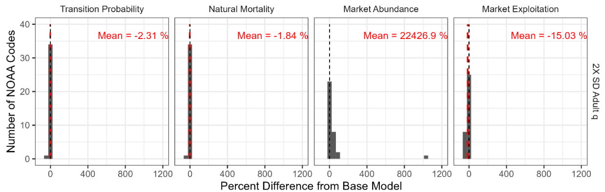
Figure 207. Results of sensitivity analyses for doubling the standard deviation (SD) of adult catchability penalty. Bars indicate frequency histogram of relative errors between the base model and sensitivity analysis for all NOAA codes. The mean relative error (over NOAA codes) is indicated by the red dashed line and no difference between the base model and sensitivity analysis is indicated by the black dashed line.
