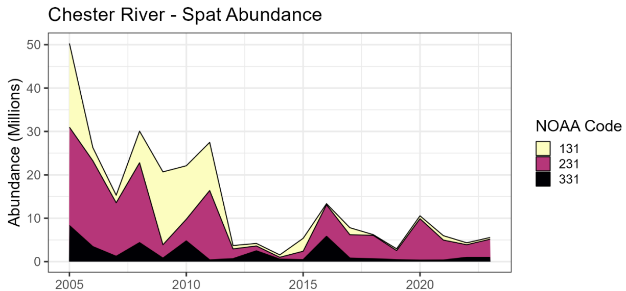
Figure 177. Estimated spat oyster abundance among modeled NOAA codes in the Chester River Region under Maryland management during 2005-2023.
