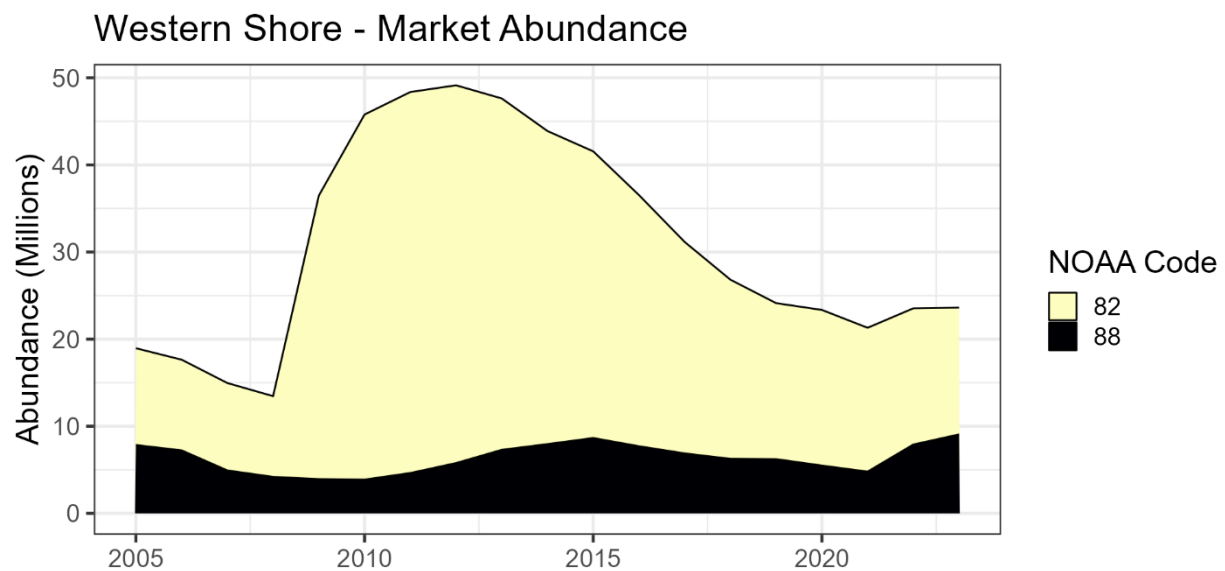
Figure 188. Estimated market oyster abundance among modeled NOAA codes in the Western Shore Region under Maryland management during 2005-2023.
