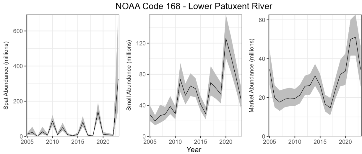
Figure 113. Estimated abundance of spat, small, and markets oysters during 2005-2023 in Lower Patuxent River. The lines indicate the estimated abundances, and the shaded areas indicate approximate 95% confidence intervals.
