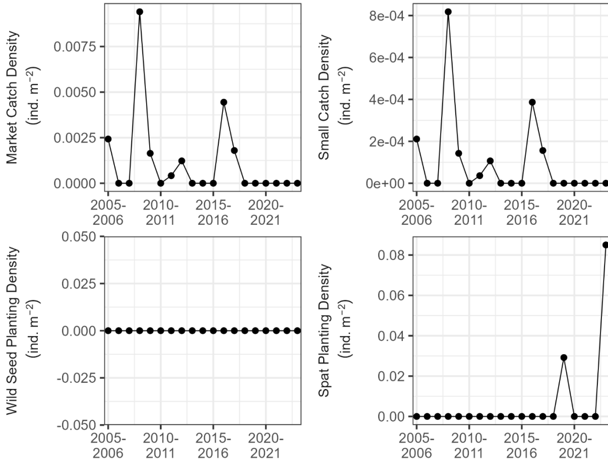
Figure 147. Catch density of market oysters, catch density of small oysters, wild seed planting density, and spat planting density during 2005-2023 in Breton & St. Clements Bay. Density was calculated as the number of individuals divided by habitat area for each data source.
