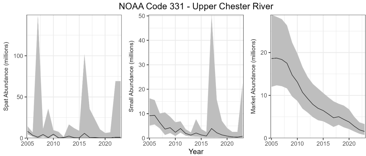
Figure 184. Estimated abundance of spat, small, and markets oysters during 2005-2023 in Upper Chester River. The lines indicate the estimated abundances, and the shaded areas indicate approximate 95% confidence intervals.
