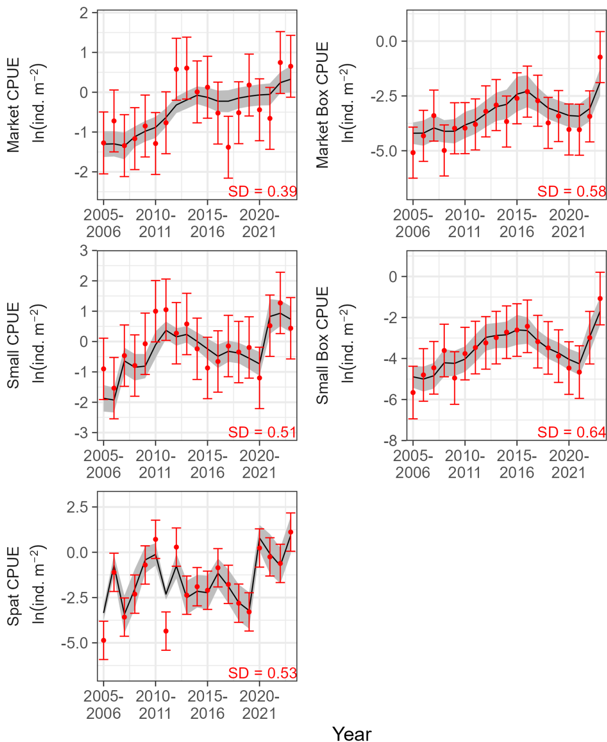
Figure 31. Estimated (line) and observed (points) values for Lower Choptank River. Variable and symbol definitions are the same as Figure 12.
