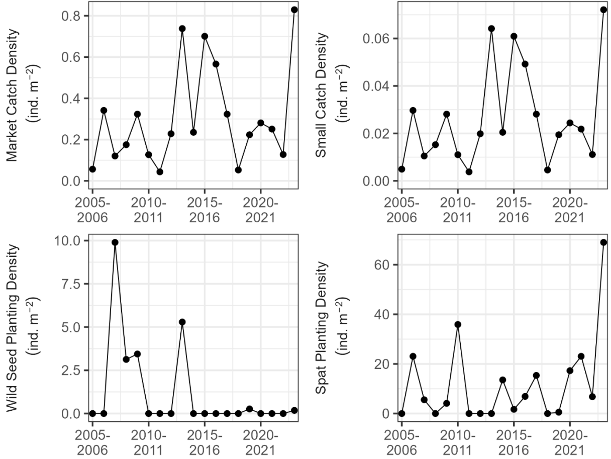
Figure 196. Catch density of market oysters, catch density of small oysters, wild seed planting density, and spat planting density during 2005-2023 in South River. Density was calculated as the number of individuals divided by habitat area for each data source.
