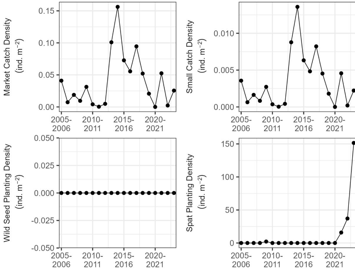
Figure 68. Catch density of market oysters, catch density of small oysters, wild seed planting density, and spat planting density during 2005-2023 in Manokin River. Density was calculated as the number of individuals divided by habitat area for each data source.
