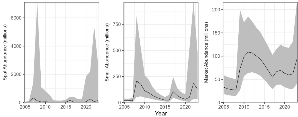
Figure 116. Estimated abundance of spat, small, and markets oysters during 2005-2023 in Mid Patuxent River. The lines indicate the estimated abundances, and the shaded areas indicate approximate 95% confidence intervals.
