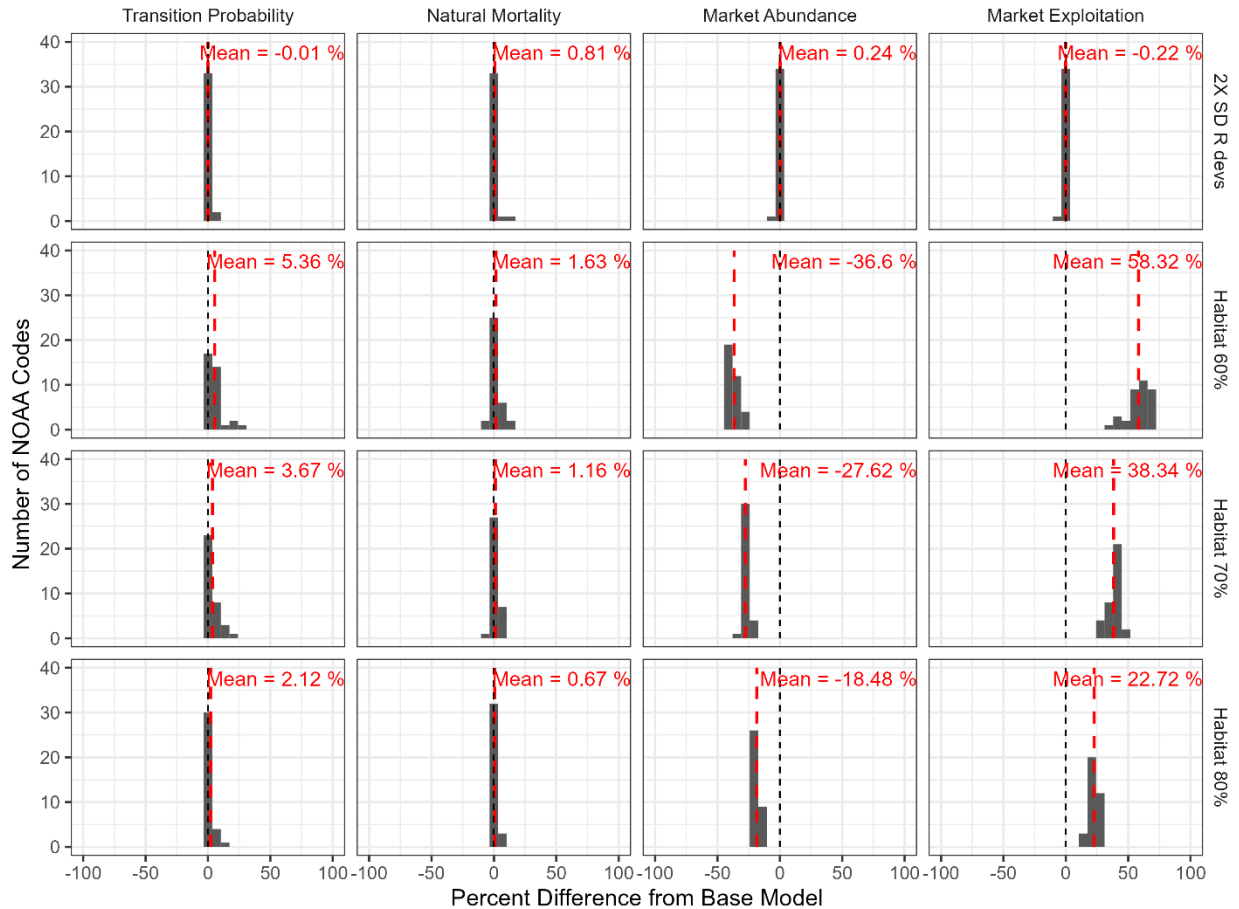
Figure 202. Results of sensitivity analyses for the mean of the standard deviation (SD) of the penalty for recruitment deviations (top row), habitat area at 60% of the base model in each NOAA code (second row), habitat area at 70% of the base model in each NOAA code (third row), and habitat area at 80% of the base model in each NOAA code (bottom row). Bars indicate frequency histogram of relative errors between the base model and sensitivity analysis for all NOAA codes. The mean relative error (over NOAA codes) is indicated by the red dashed line and no difference between the base model and sensitivity analysis is indicated by the black dashed line.
