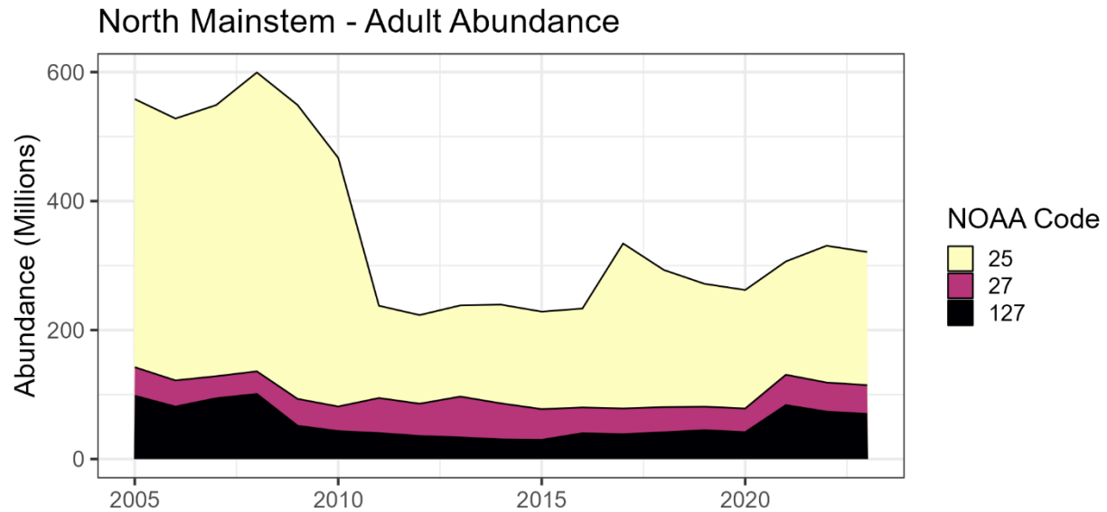
Figure 151. Estimated adult oyster abundance among modeled NOAA codes in the North Mainstem Region under Maryland management during 2005-2023.
