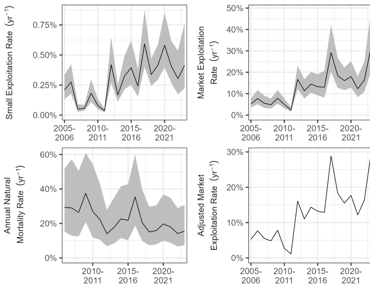
Figure 140. Estimated small exploitation rate, market exploitation rate, annual natural mortality rate, and adjusted market exploitation rate during 2005-2023 in St. Mary's River. The shaded areas indicate approximate 95% confidence intervals.
