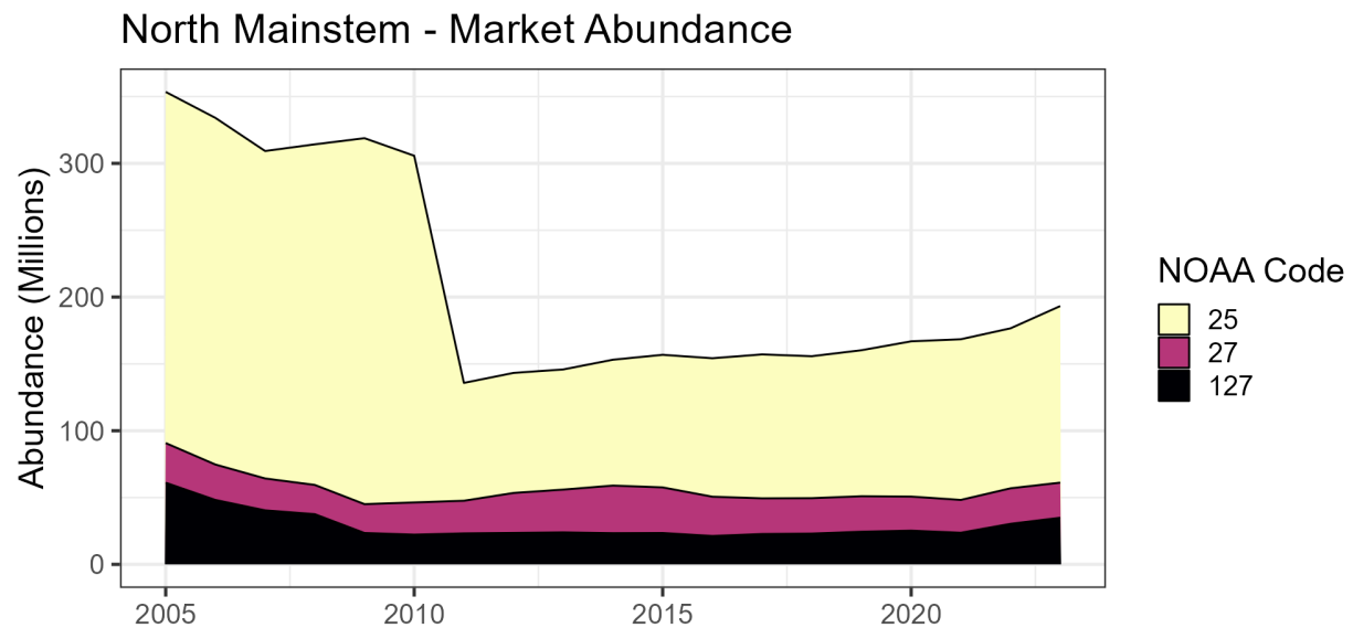
Figure 152. Estimated market oyster abundance among modeled NOAA codes in the North Mainstem Region under Maryland management during 2005-2023.
