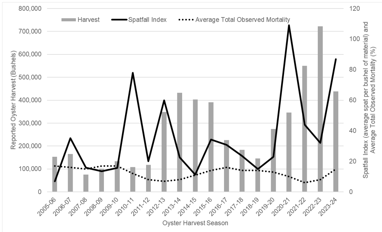
Figure 5. Oyster harvest from the Maryland portion of Chesapeake Bay along with an index of spatfall and mortality from the Maryland Department of Natural Resources fall dredge survey.
