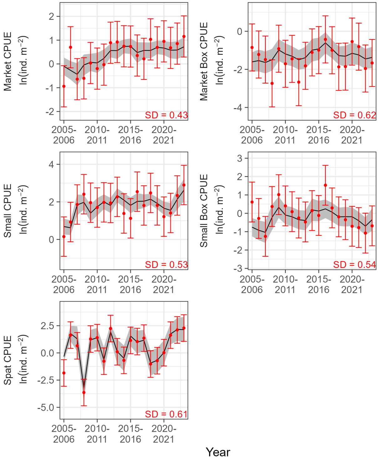
Figure 22. Estimated (line) and observed (points) values for St. Mary's River. Variable and symbol definitions are the same as Figure 12.
