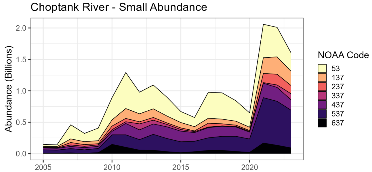
Figure 86. Estimated small oyster abundance among modeled NOAA codes in the Choptank River Region under Maryland management during 2005-2023.
