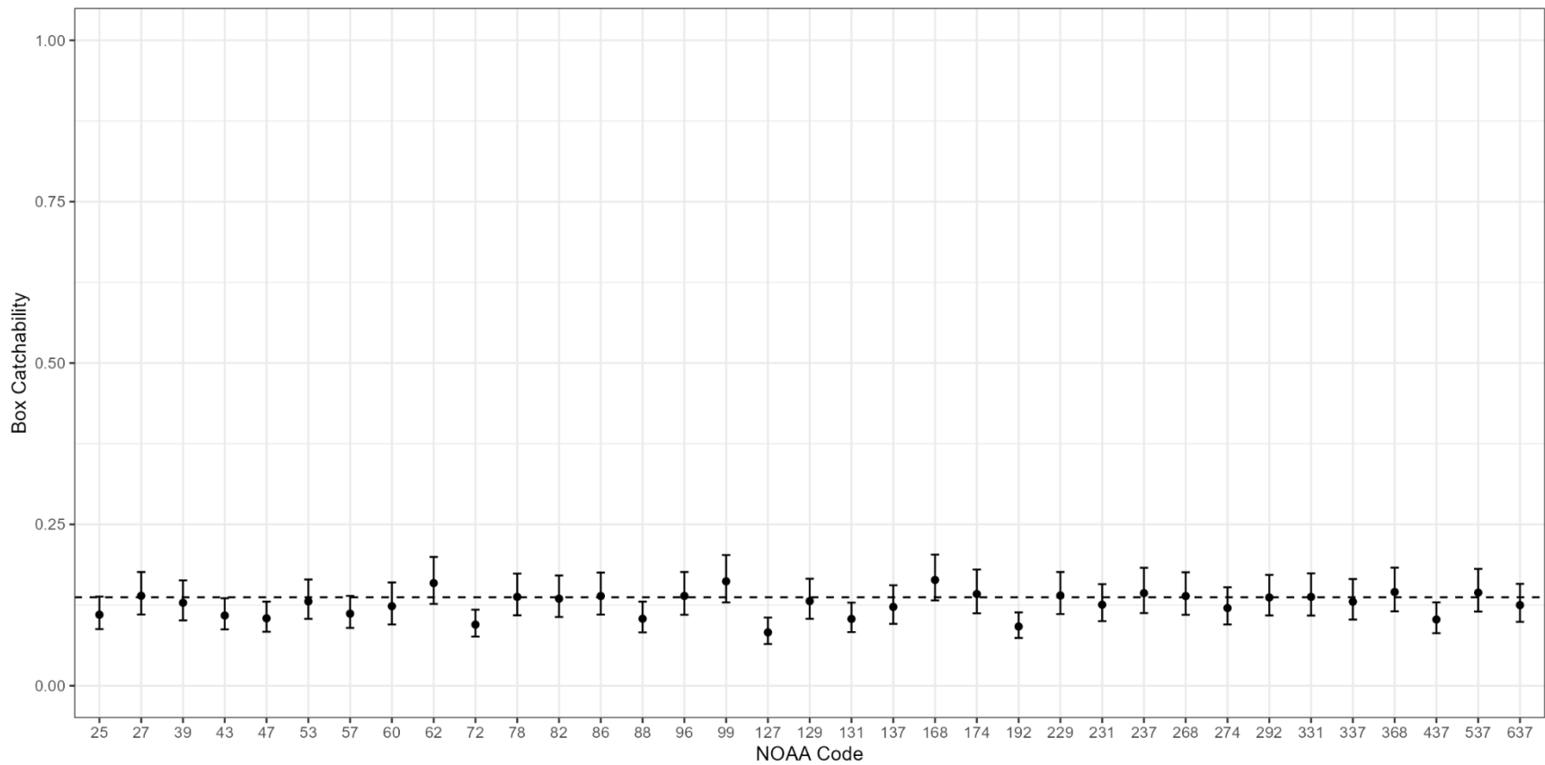
Figure 50. Estimated box (small and market) catchability in each NOAA code (points) with approximate 95% confidence intervals (whiskers). The dashed line represents the median of the penalty included in the model.
