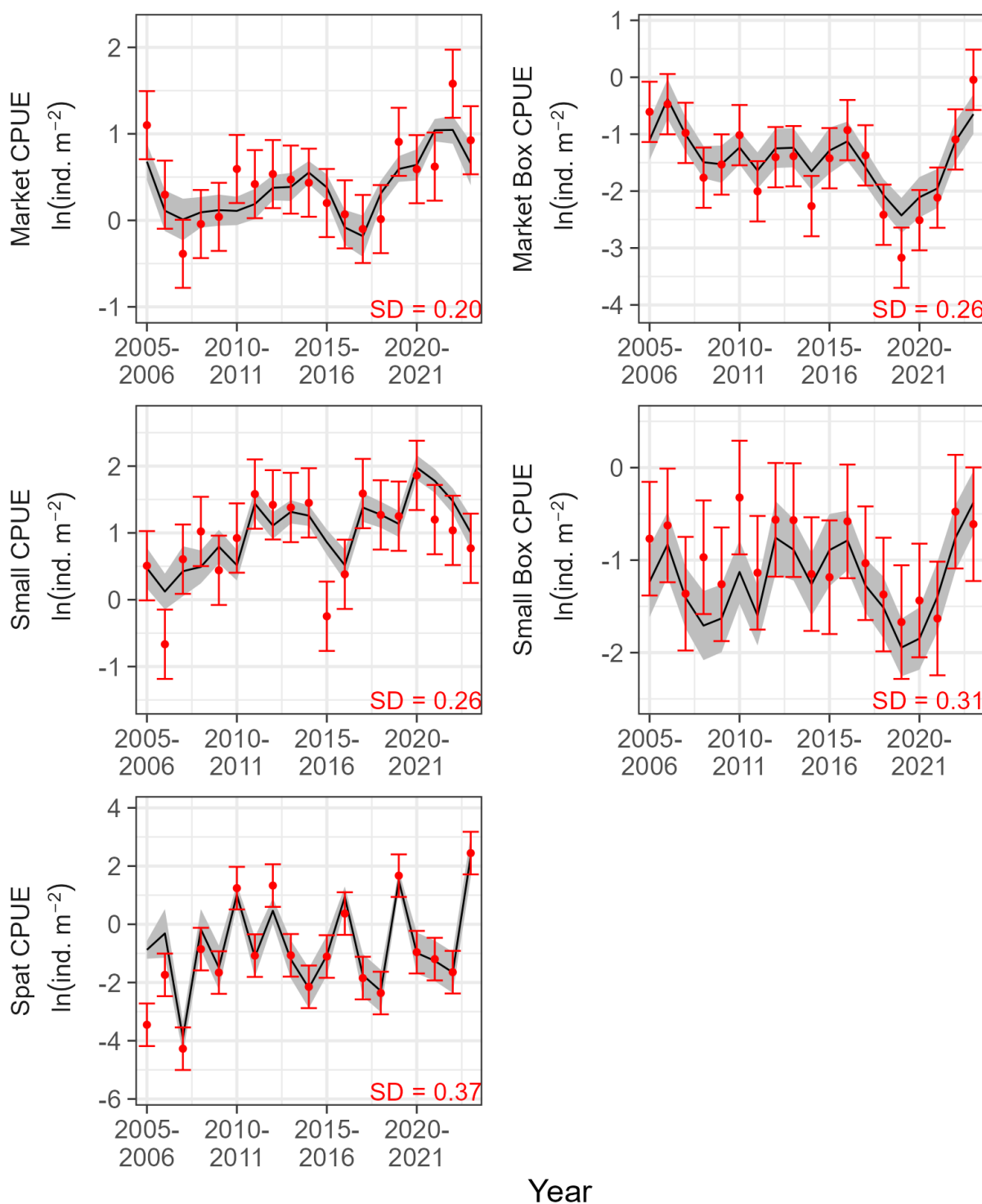
Figure 32. Estimated (line) and observed (points) values for Lower Patuxent River. Variable and symbol definitions are the same as Figure 12.
