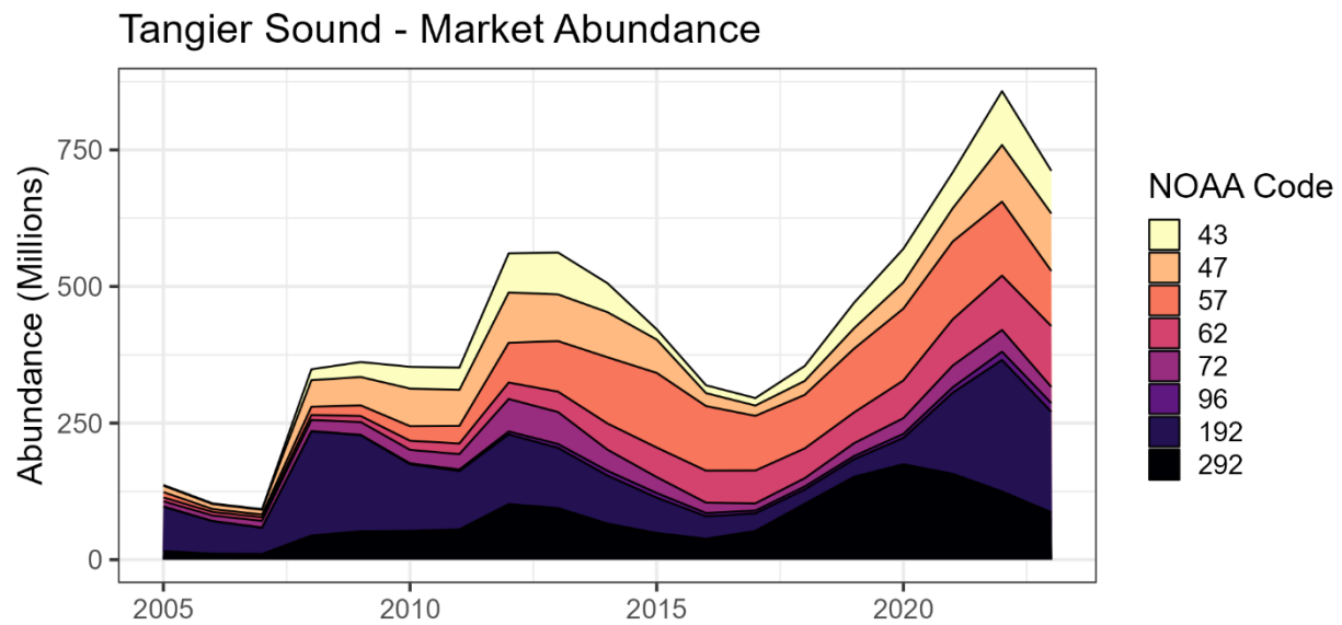
Figure 57. Estimated market oyster abundance among modeled NOAA codes in the Tangier Sound Region under Maryland management during 2005-2023.
