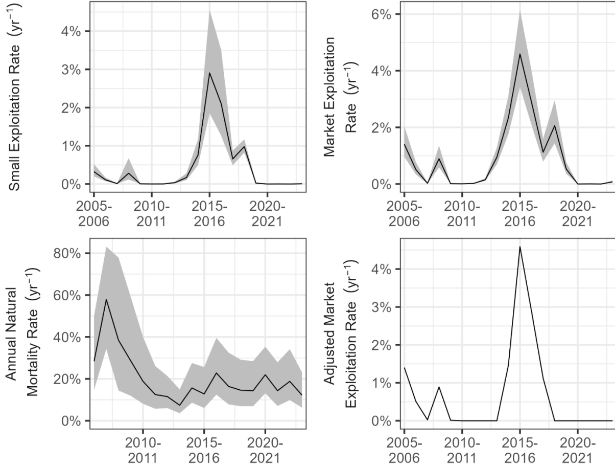
Figure 130. Estimated small exploitation rate, market exploitation rate, annual natural mortality rate, and adjusted market exploitation rate during 2005-2023 in Miles River. The shaded areas indicate approximate 95% confidence intervals.
