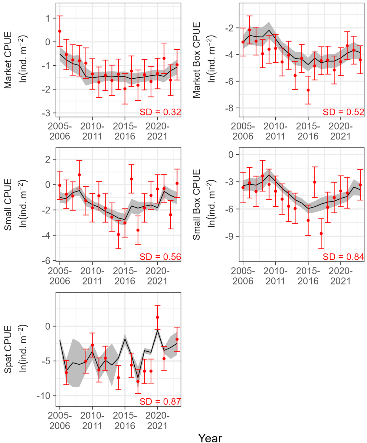
Figure 28. Estimated (line) and observed (points) values for North Mid-Bay. Variable and symbol definitions are the same as Figure 12.
