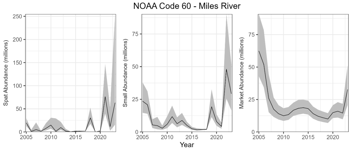
Figure 129. Estimated abundance of spat, small, and markets oysters during 2005-2023 in Miles River. The lines indicate the estimated abundances, and the shaded areas indicate approximate 95% confidence intervals.
