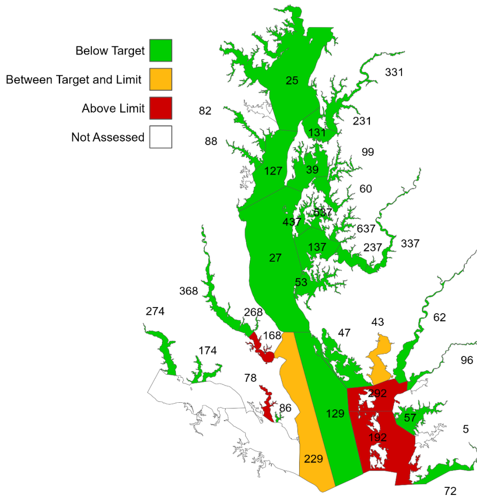
Figure 199. Status of each NOAA Code relative to the exploitation rate reference points.
