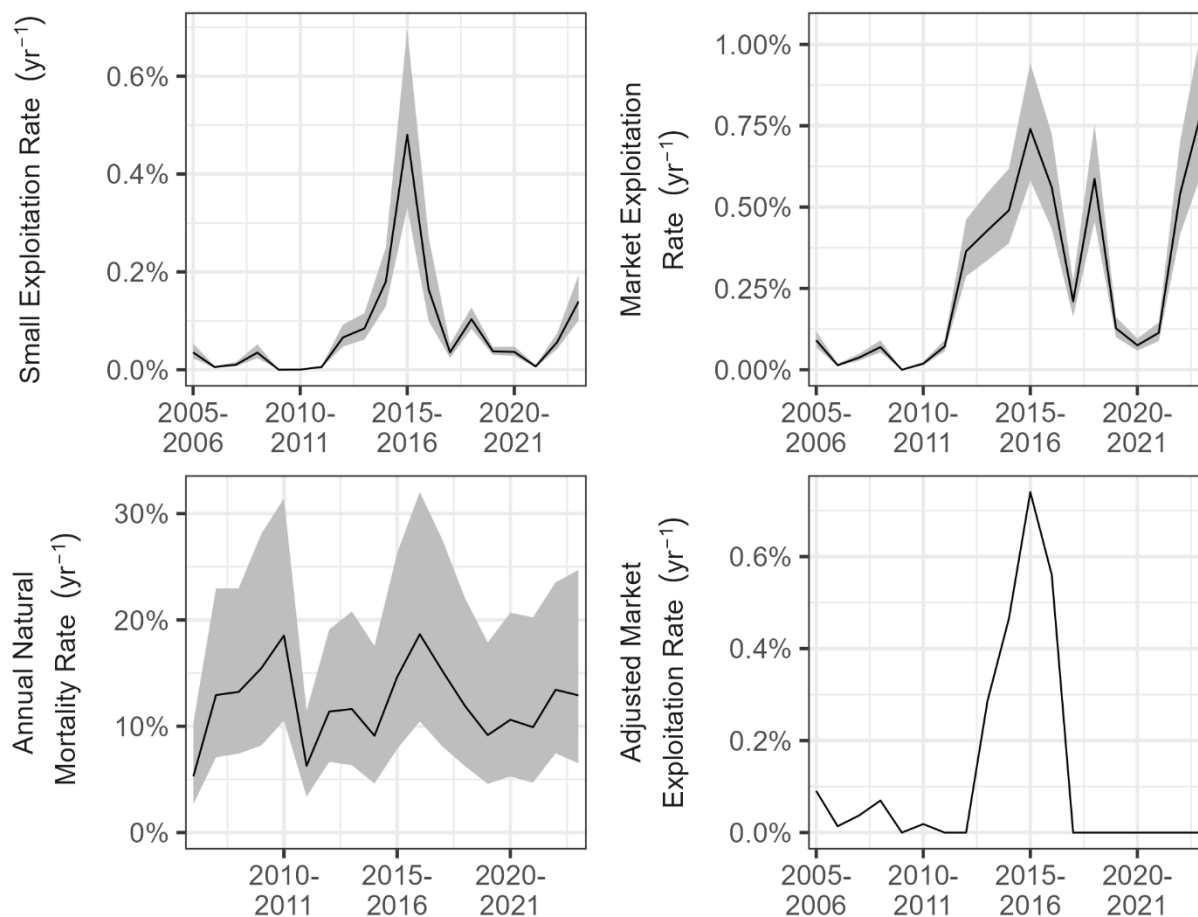
Figure 107. Estimated small exploitation rate, market exploitation rate, annual natural mortality rate, and adjusted market exploitation rate during 2005-2023 in Tred Avon River. The shaded areas indicate approximate 95% confidence intervals.
