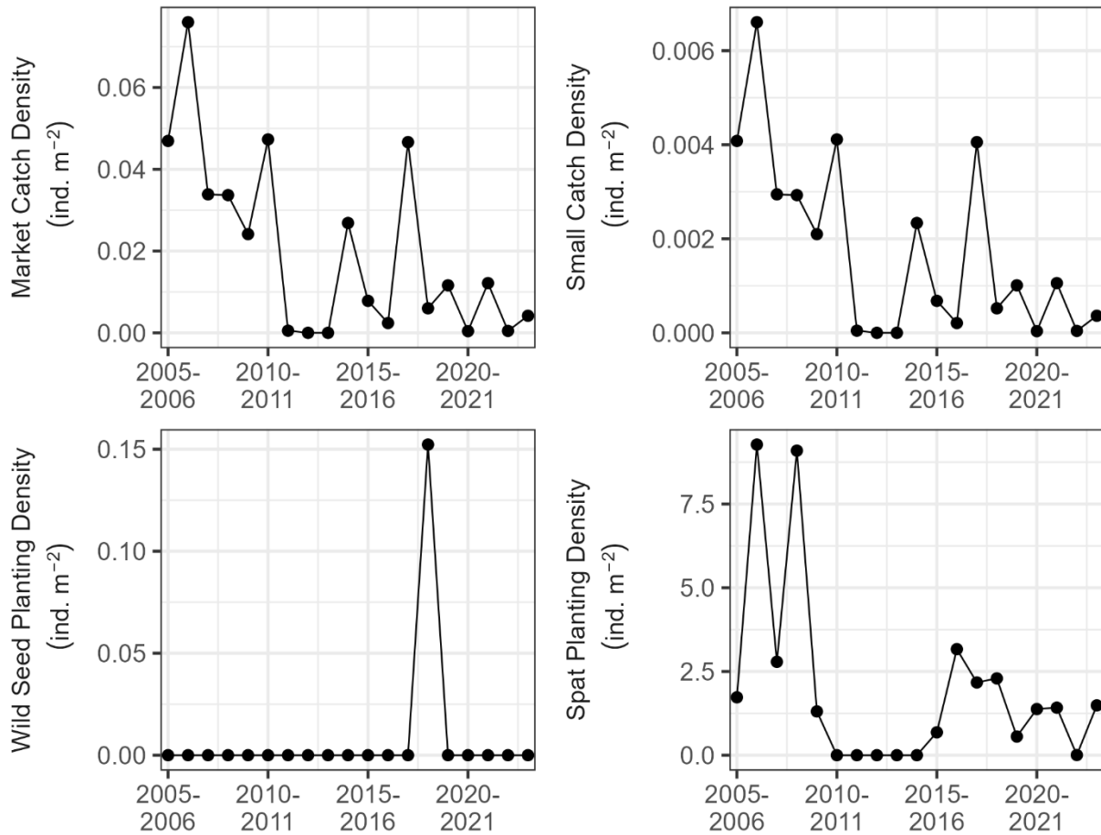
Figure 183. Catch density of market oysters, catch density of small oysters, wild seed planting density, and spat planting density during 2005-2023 in Mid Chester River. Density was calculated as the number of individuals divided by habitat area for each data source.
