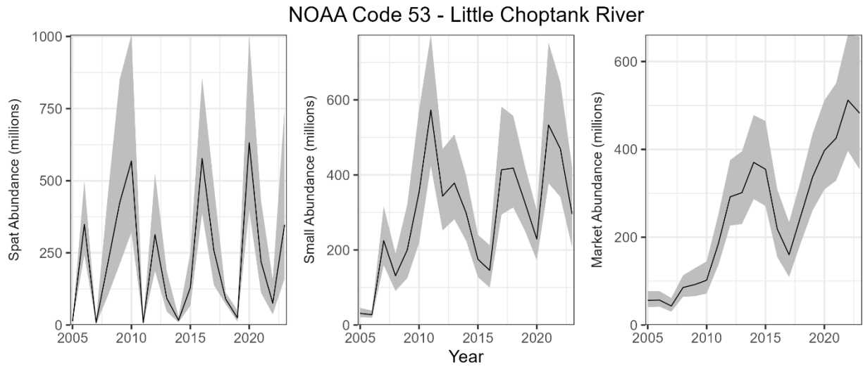
Figure 88. Estimated abundance of spat, small, and markets oysters during 2005-2023 in Little Choptank River. The lines indicate the estimated abundances, and the shaded areas indicate approximate 95% confidence intervals.
