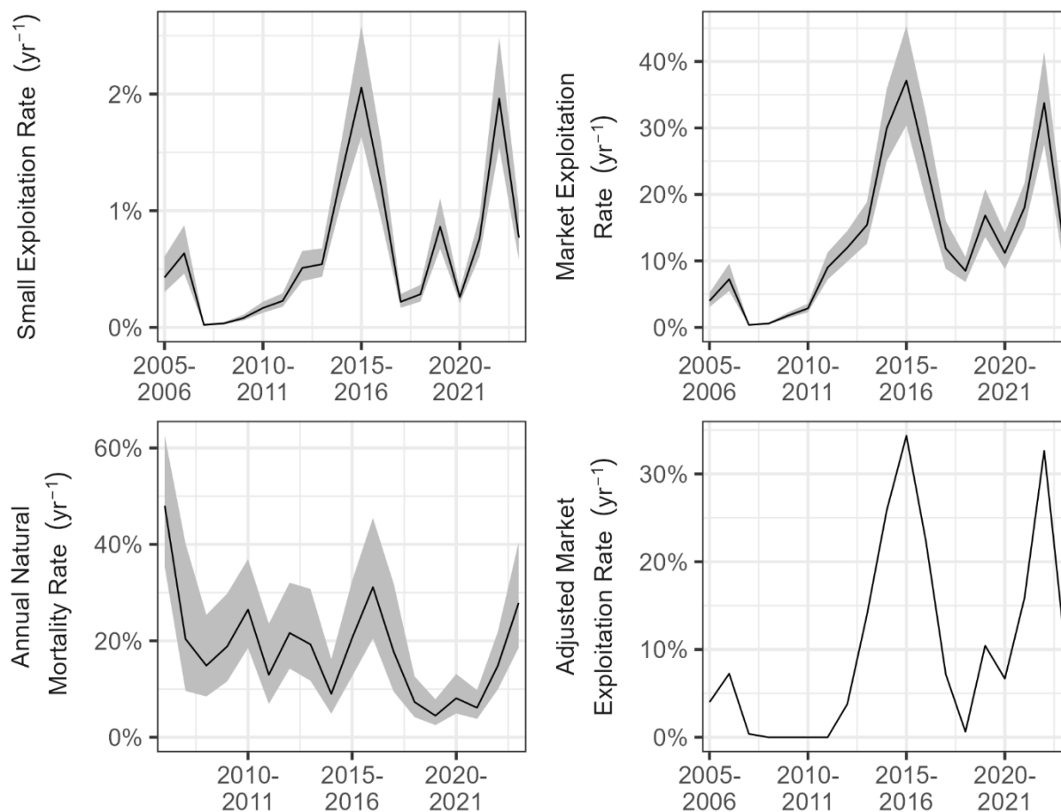
Figure 114. Estimated small exploitation rate, market exploitation rate, annual natural mortality rate, and adjusted market exploitation rate during 2005-2023 in Lower Patuxent River. The shaded areas indicate approximate 95% confidence intervals.
