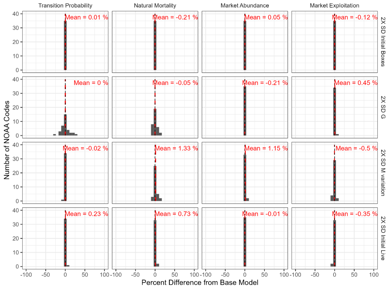
Figure 201. Results of sensitivity analyses for the mean of the standard deviation (SD) of the penalty for the initial abundance of boxes (top row), the standard deviation (SD) of the penalty on the transition probability (G) (second row), the standard deviation (SD) of the penalty for variation in natural mortality within NOAA codes over time (third row), the standard deviation (SD) of the penalty on initial abundance of live small and market oysters (bottom row). Bars indicate frequency histogram of relative errors between the base model and sensitivity analysis for all NOAA codes. The mean relative error (over NOAA codes) is indicated by the red dashed line and no difference between the base model and sensitivity analysis is indicated by the black dashed line.
