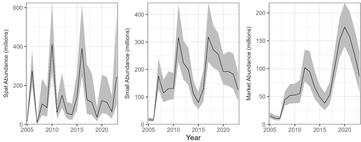
Figure 81. Estimated abundance of spat, small, and markets oysters during 2005-2023 in Tangier Sound North. The lines indicate the estimated abundances, and the shaded areas indicate approximate 95% confidence intervals.
