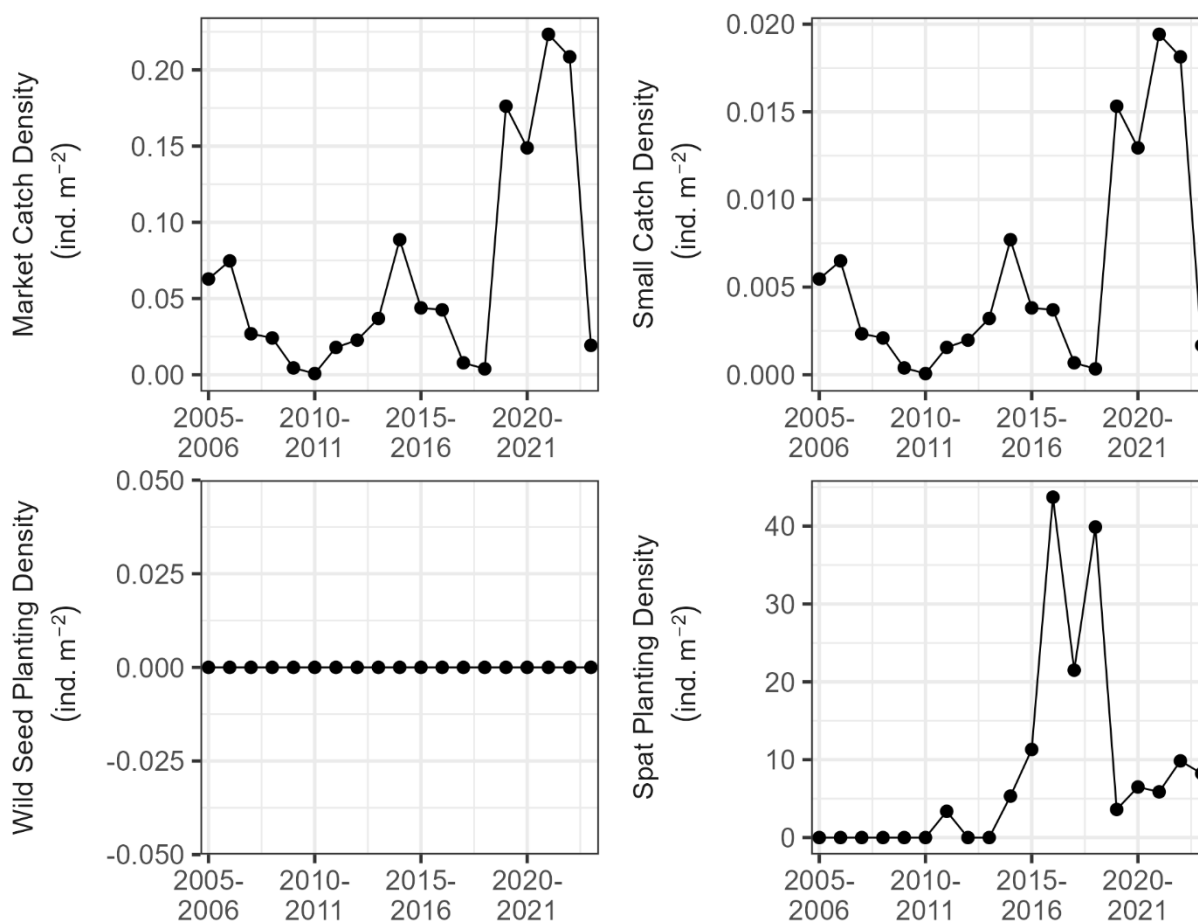
Figure 90. Catch density of market oysters, catch density of small oysters, wild seed planting density, and spat planting density during 2005-2023 in Little Choptank River. Density was calculated as the number of individuals divided by habitat area for each data source.
