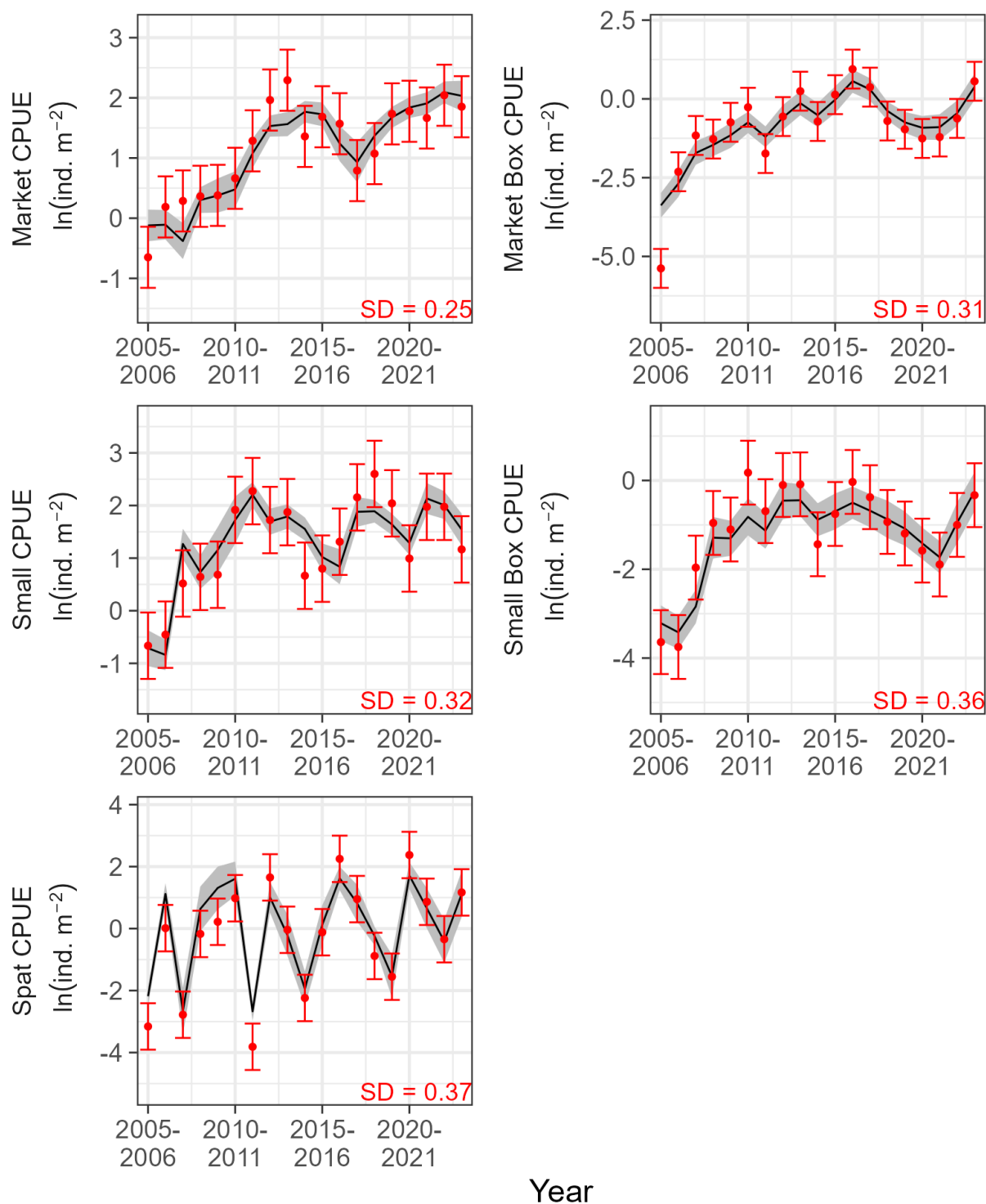
Figure 17. Estimated (line) and observed (points) values for the Little Choptank River. Variable and symbol definitions are the same as Figure 12.
