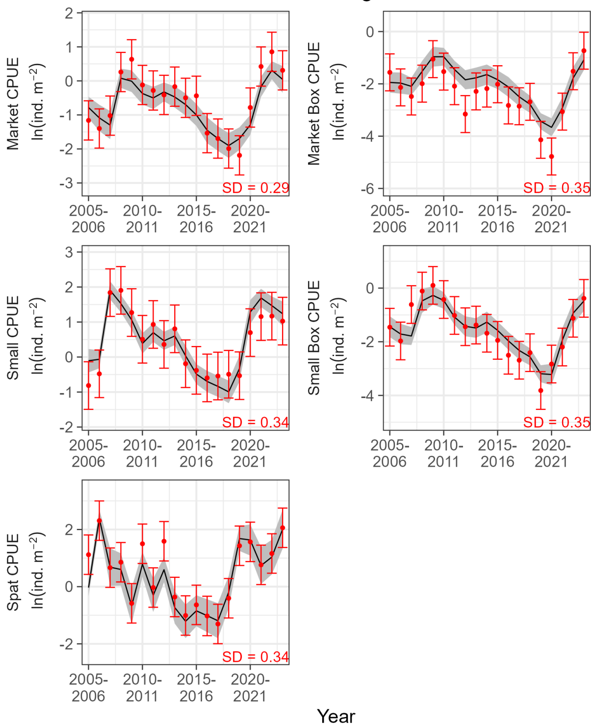
Figure 34. Estimated (line) and observed (points) values for Tangier Sound South. Variable and symbol definitions are the same as Figure 12.
