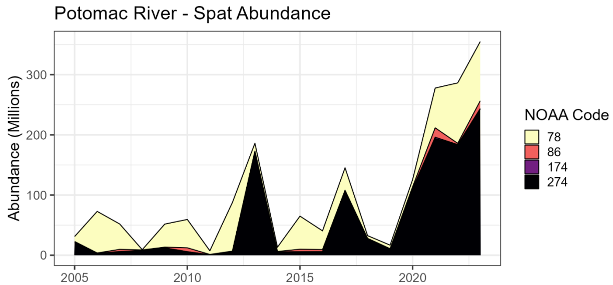
Figure 138. Estimated spat oyster abundance among modeled NOAA codes in the Potomac River Region under Maryland management during 2005-2023.
