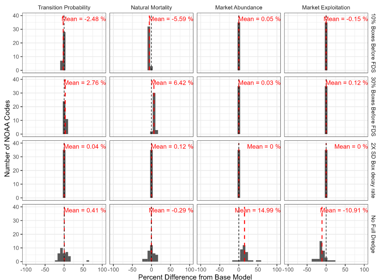
Figure 200. Results of sensitivity analyses for 10% of boxes not available to the Fall Dredge Survey (FDS; top row), 30% of boxes not available to the FDS (second row), doubling the prior standard deviation (SD) of the box decay rate (third row), and removing full dredge tows from Fall Survey data (bottom row). Bars indicate frequency histogram of relative errors between the base model and sensitivity analysis for all NOAA codes. The mean relative error (over NOAA codes) is indicated by the red dashed line and no difference between the base model and sensitivity analysis is indicated by the black dashed line.
