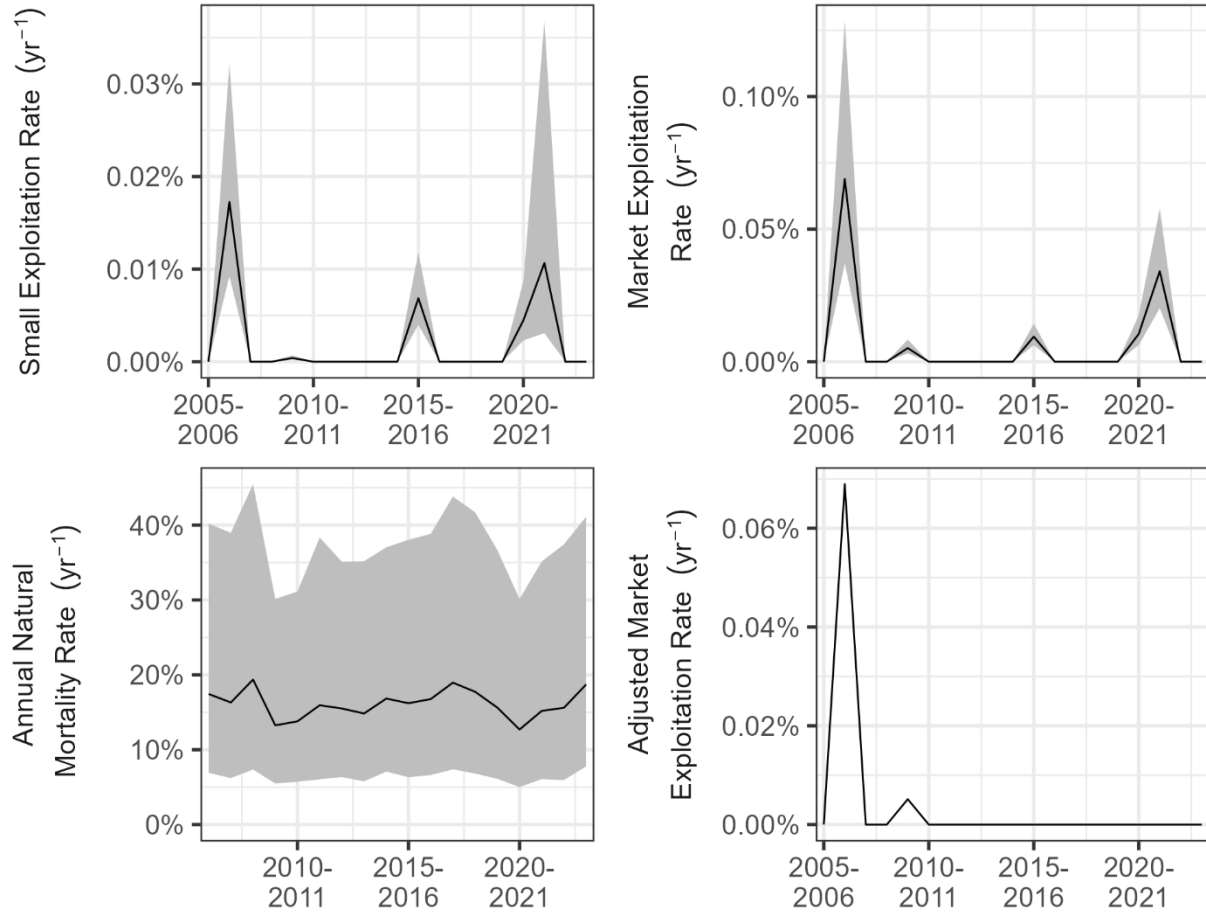
Figure 192. Estimated small exploitation rate, market exploitation rate, annual natural mortality rate, and adjusted market exploitation rate during 2005-2023 in Severn River. The shaded areas indicate approximate 95% confidence intervals.
