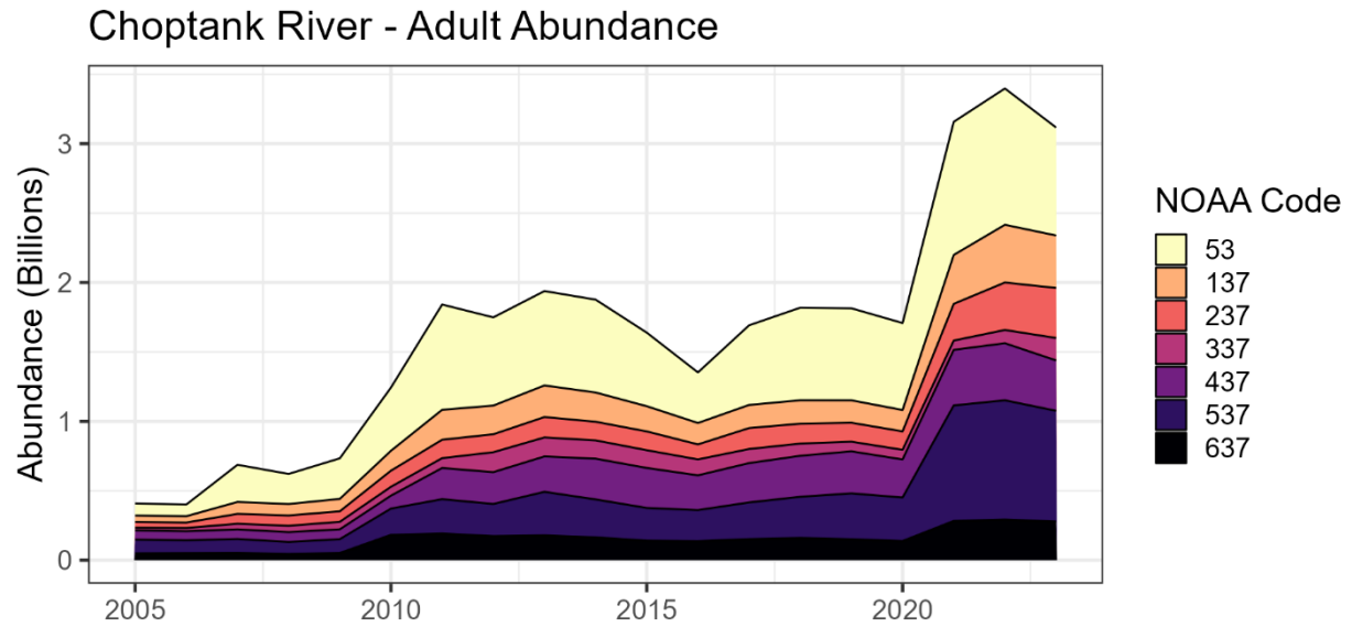
Figure 84. Estimated adult oyster abundance among modeled NOAA codes in the Choptank River Region under Maryland management during 2005-2023.
