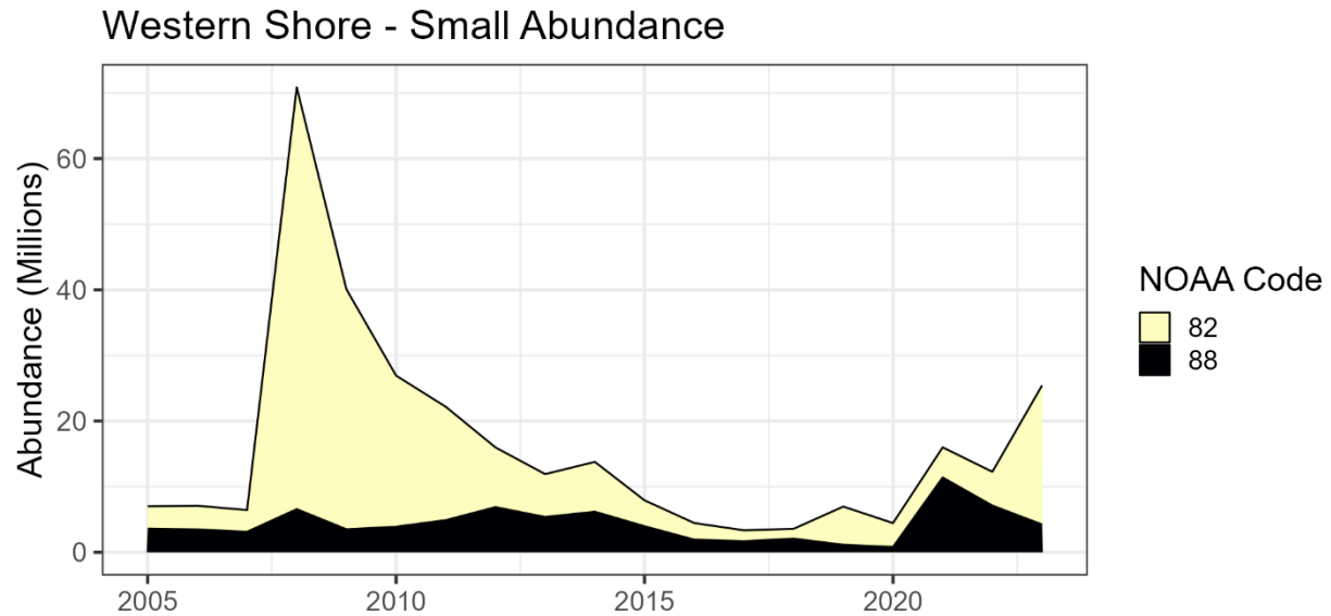
Figure 189. Estimated small oyster abundance among modeled NOAA codes in the Western Shore Region under Maryland management during 2005-2023.
