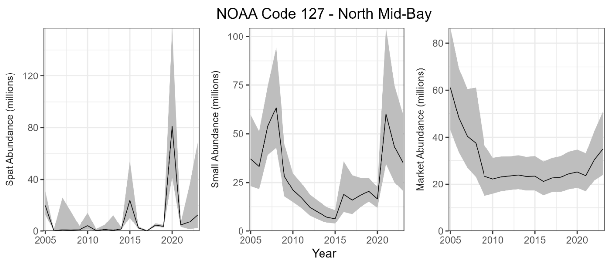
Figure 161. Estimated abundance of spat, small, and markets oysters during 2005-2023 in North Mid-Bay. The lines indicate the estimated abundances, and the shaded areas indicate approximate 95% confidence intervals.
