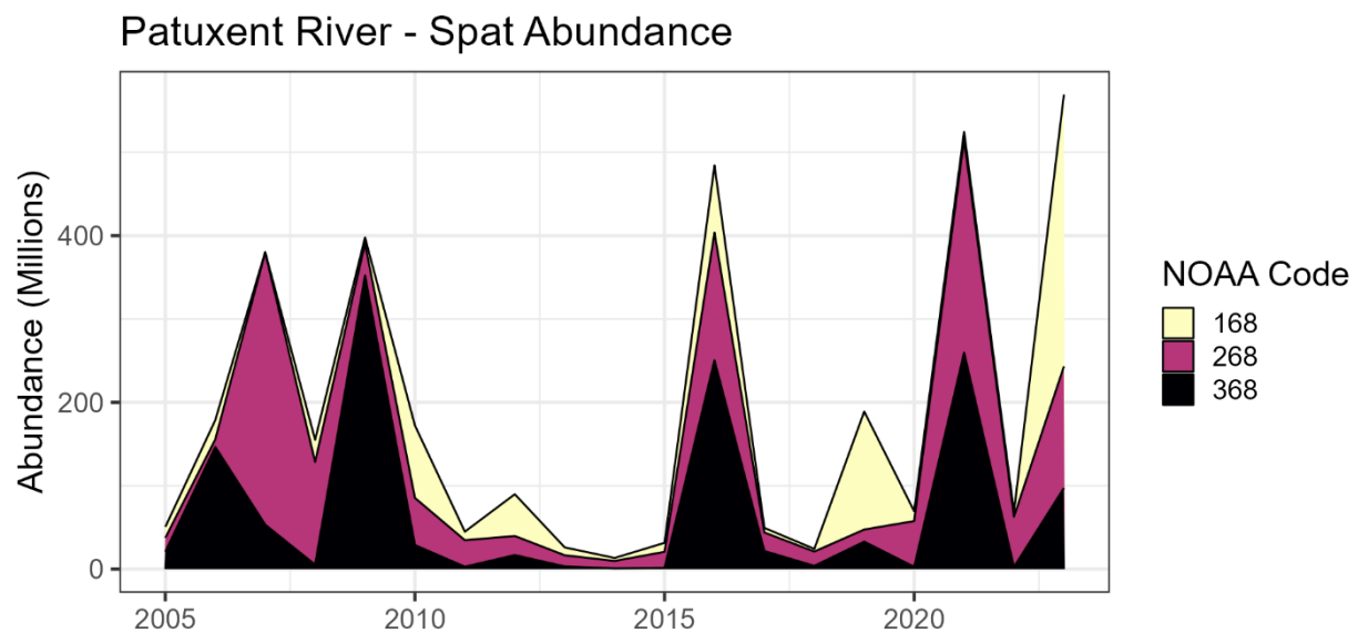
Figure 112. Estimated spat oyster abundance among modeled NOAA codes in the Patuxent River Region under Maryland management during 2005-2023.
