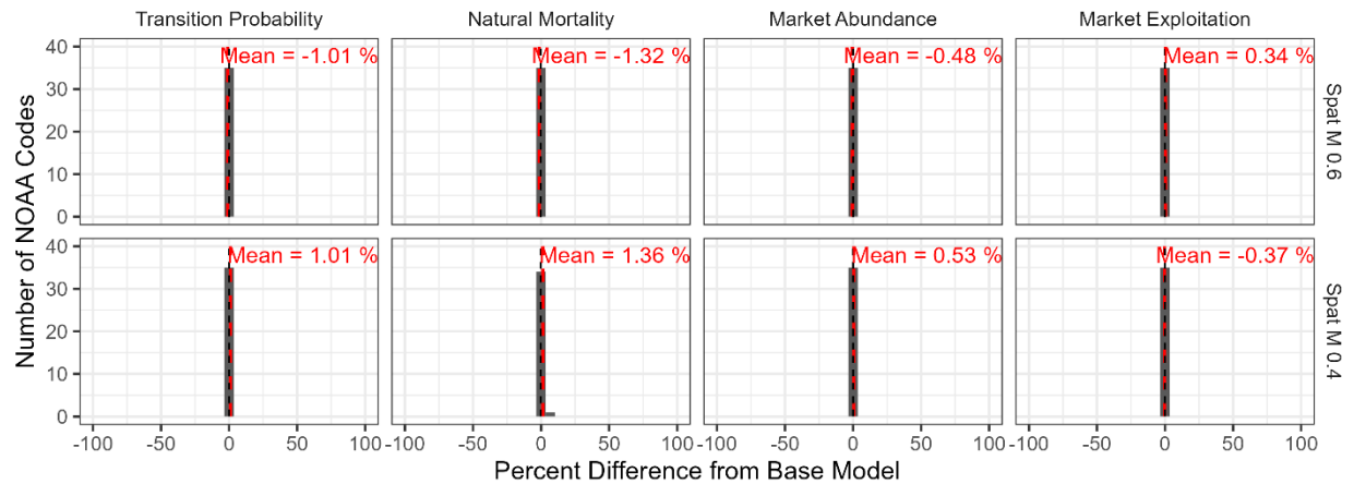
Figure 205. Results of sensitivity analyses for 0.6 instantaneous natural mortality rate for spat (top row), 0.4 instantaneous natural mortality rate for spat (bottom row). Bars indicate frequency histogram of relative errors between the base model and sensitivity analysis for all NOAA codes. The mean relative error (over NOAA codes) is indicated by the red dashed line and no difference between the base model and sensitivity analysis is indicated by the black dashed line.
