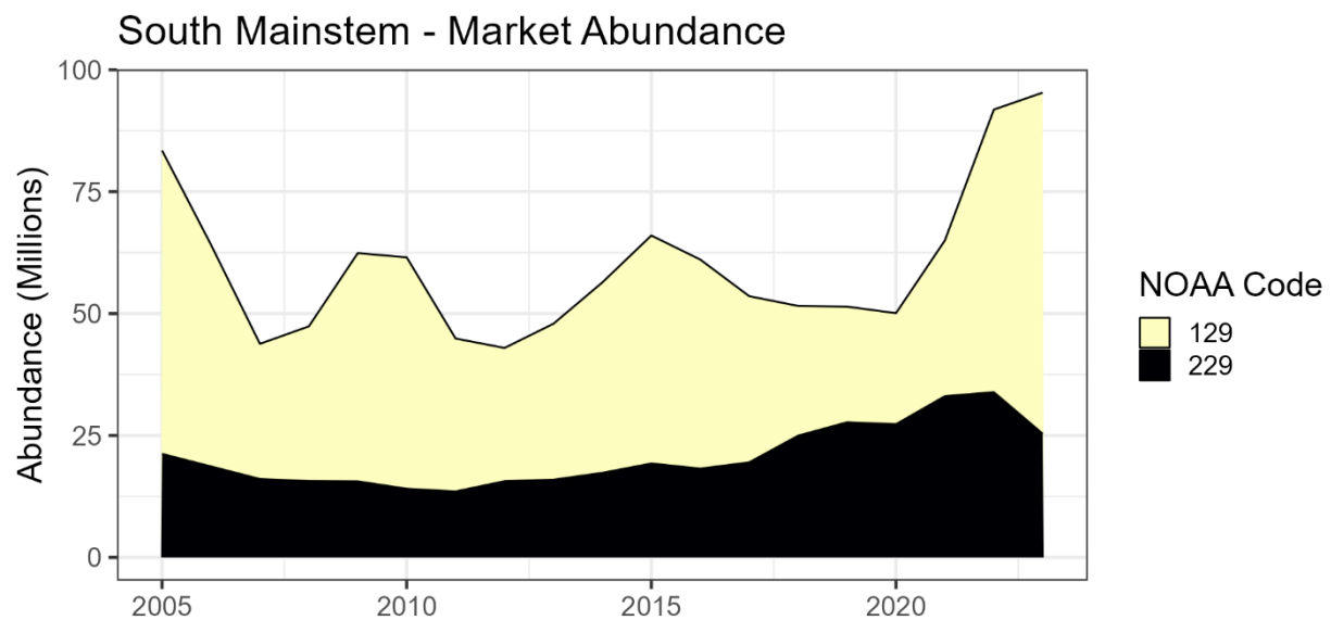
Figure 165. Estimated market oyster abundance among modeled NOAA codes in the South Mainstem Region under Maryland management during 2005-2023.
