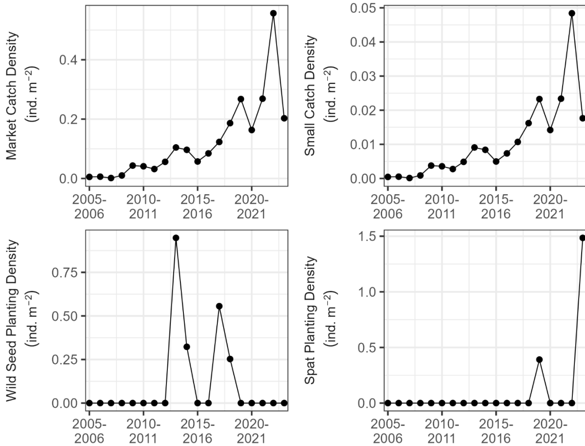
Figure 173. Catch density of market oysters, catch density of small oysters, wild seed planting density, and spat planting density during 2005-2023 in Lower Bay West. Density was calculated as the number of individuals divided by habitat area for each data source.
