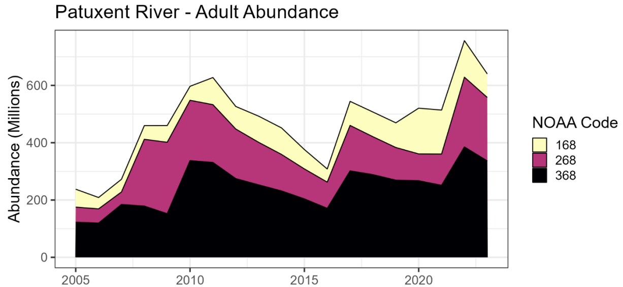
Figure 109. Estimated adult oyster abundance among modeled NOAA codes in the Patuxent River Region under Maryland management during 2005-2023.
