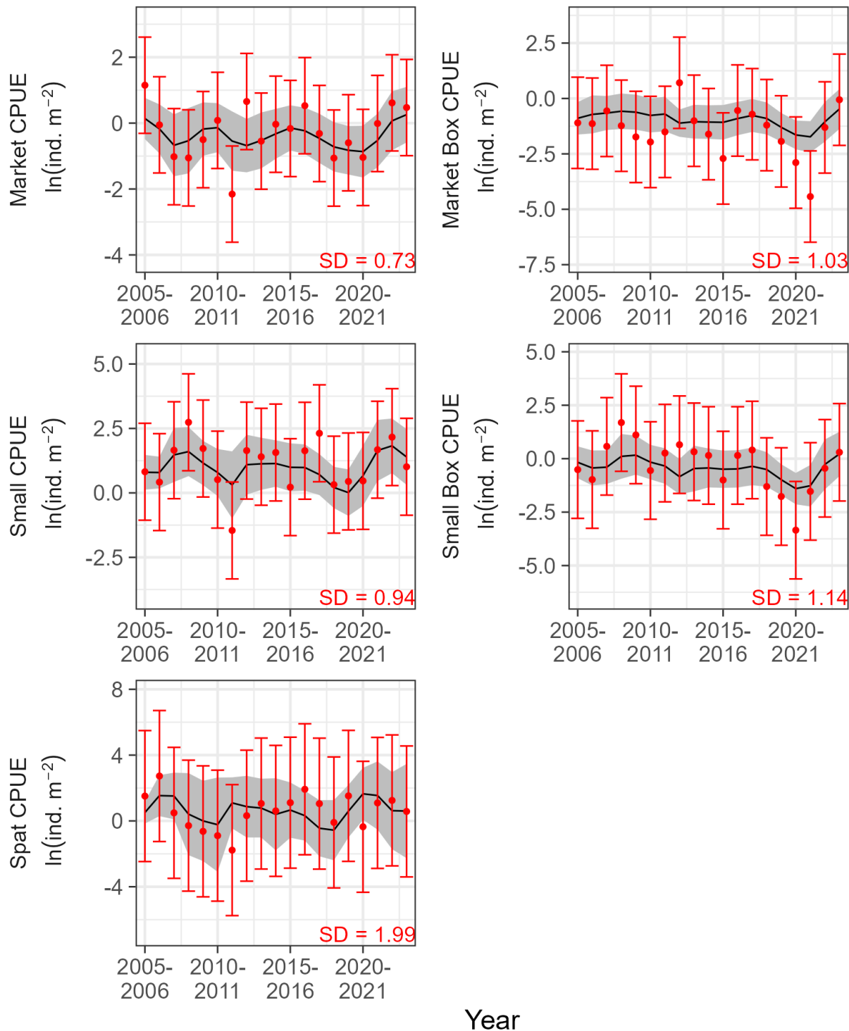
Figure 29. Estimated (line) and observed (points) values for Lower Bay East. Variable and symbol definitions are the same as Figure 12.
