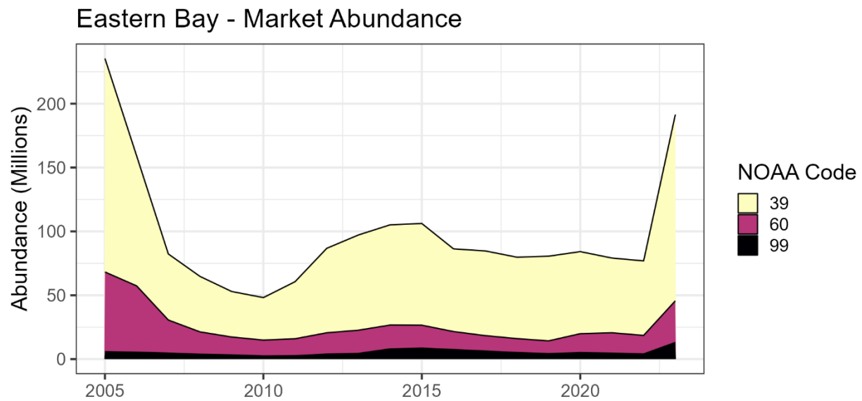
Figure 123. Estimated market oyster abundance among modeled NOAA codes in the Eastern Bay Region under Maryland management during 2005-2023.
