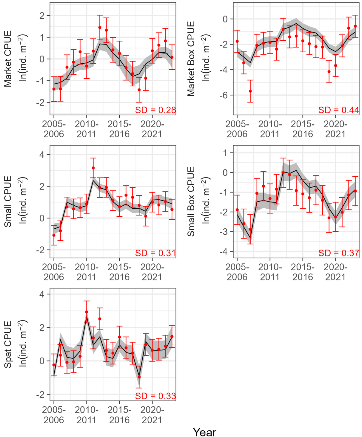
Figure 21. Estimated (line) and observed (points) values for Pocomoke Sound (NOAA code 72). Variable and symbol definitions are the same as Figure 12.
