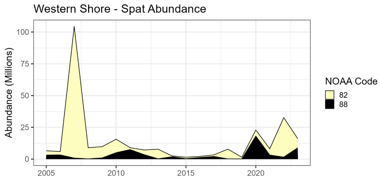
Figure 190. Estimated spat oyster abundance among modeled NOAA codes in the Western Shore Region under Maryland management during 2005-2023.
