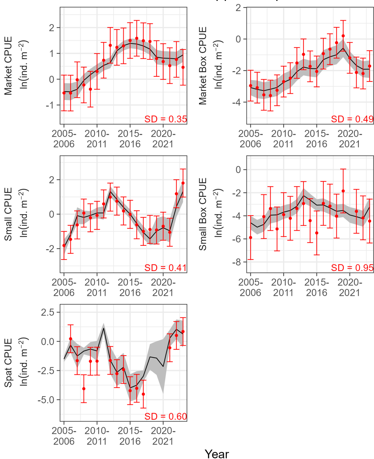
Figure 42. Estimated (line) and observed (points) values for Upper Choptank River. Variable and symbol definitions are the same as Figure 12.
