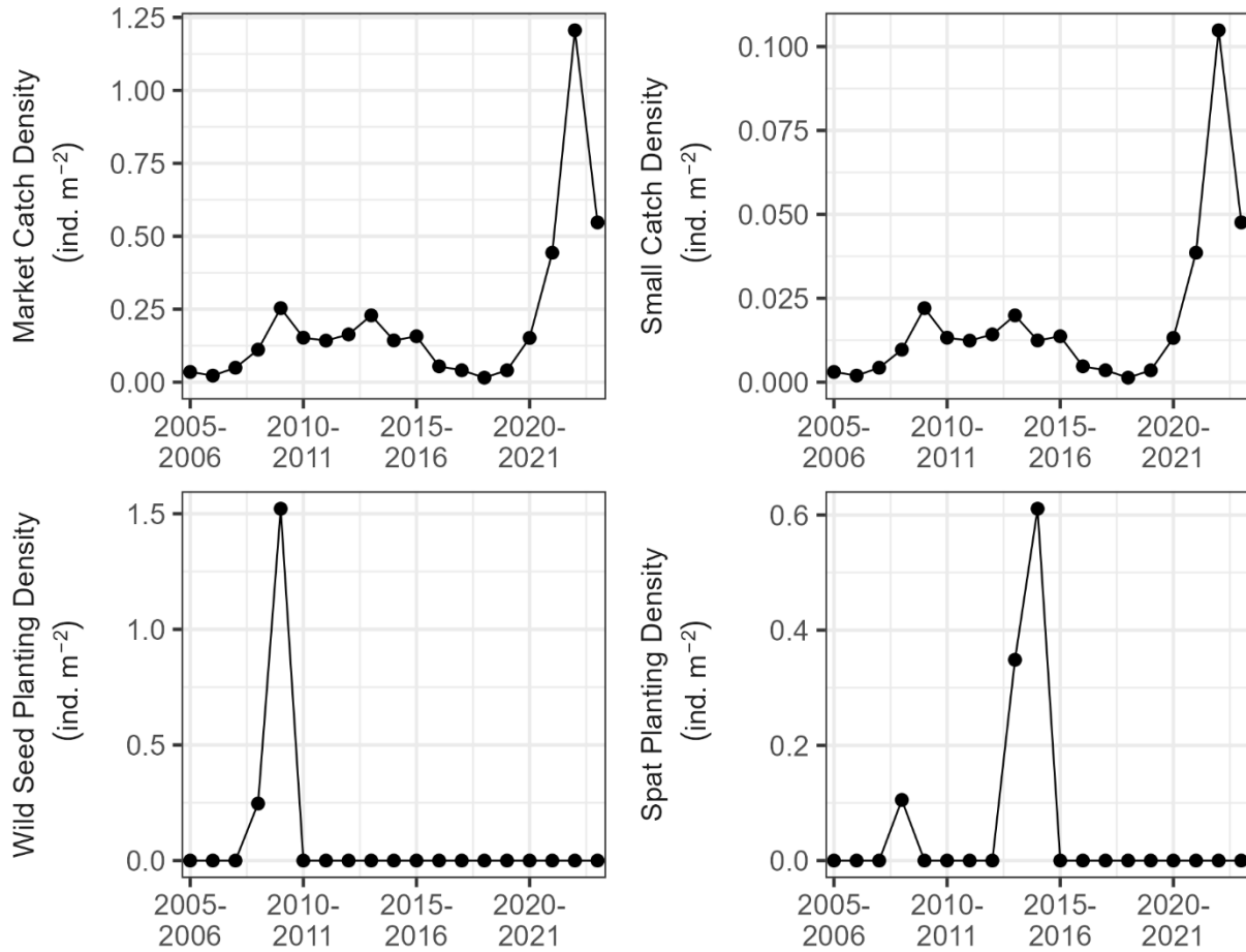
Figure 80. Catch density of market oysters, catch density of small oysters, wild seed planting density, and spat planting density during 2005-2023 in Tangier Sound South. Density was calculated as the number of individuals divided by habitat area for each data source.
