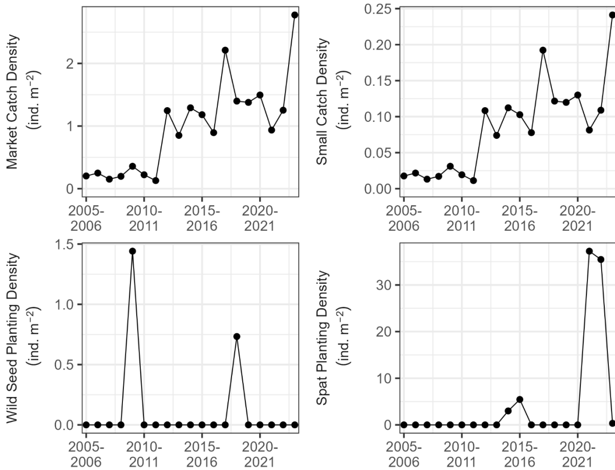
Figure 141. Catch density of market oysters, catch density of small oysters, wild seed planting density, and spat planting density during 2005-2023 in St. Mary's River. Density was calculated as the number of individuals divided by habitat area for each data source.
