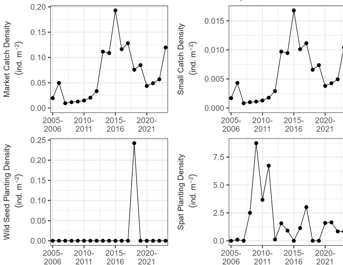
Figure 96. Catch density of market oysters, catch density of small oysters, wild seed planting density, and spat planting density during 2005-2023 in Mid Choptank River. Density was calculated as the number of individuals divided by habitat area for each data source.
