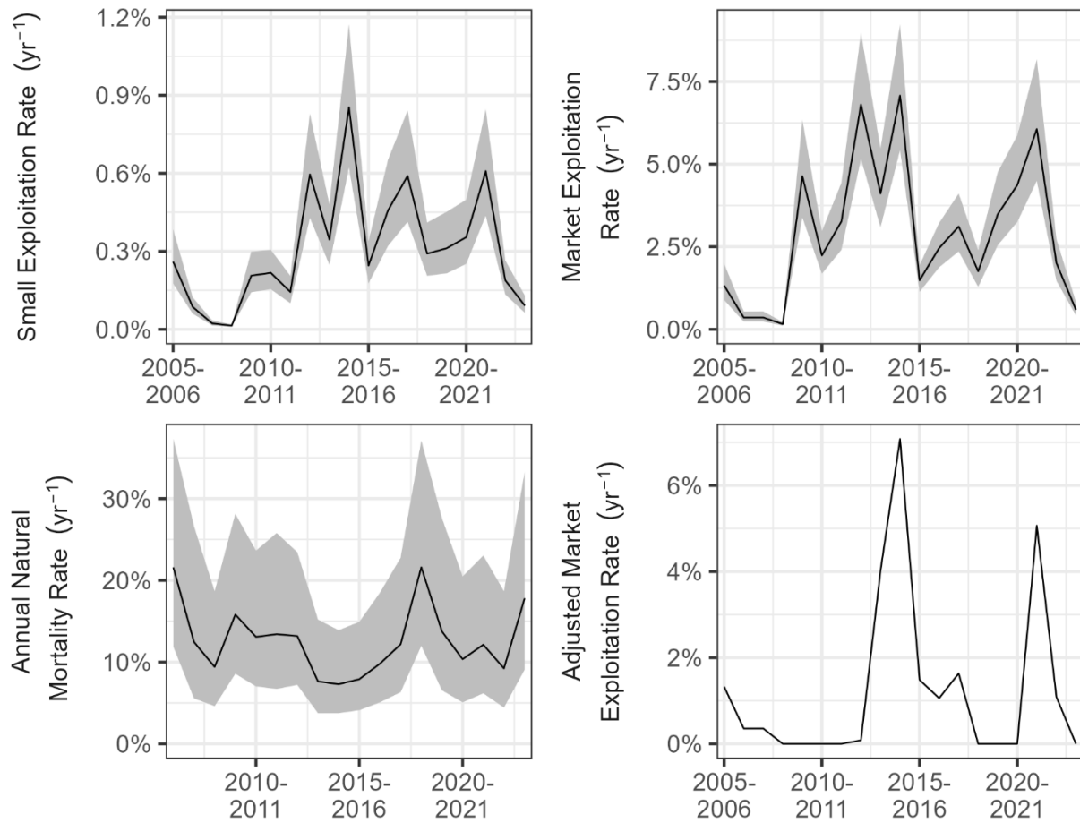
Figure 70. Estimated small exploitation rate, market exploitation rate, annual natural mortality rate, and adjusted market exploitation rate during 2005-2023 in Nanticoke River. The shaded areas indicate approximate 95% confidence intervals.
