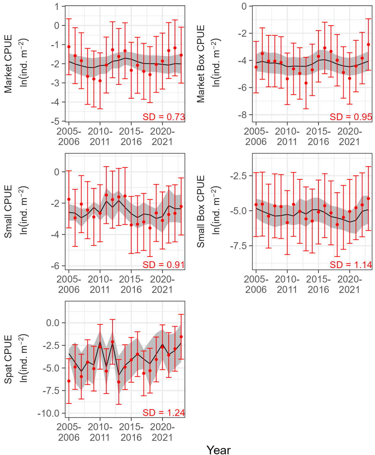
Figure 13. Estimated (line) and observed (points) values for South Mid-Bay. Variable and symbol definitions are the same as Figure 12.
