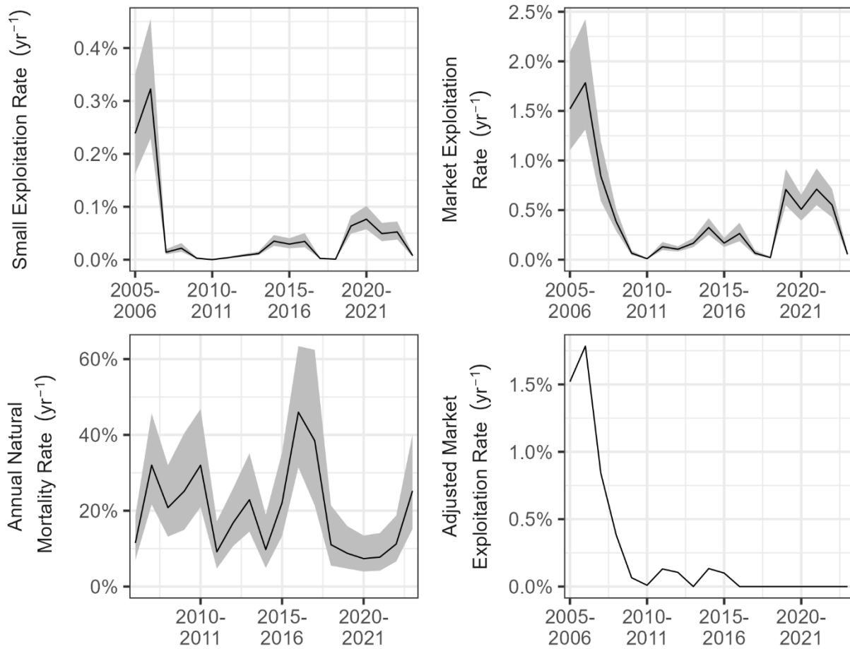
Figure 89. Estimated small exploitation rate, market exploitation rate, annual natural mortality rate, and adjusted market exploitation rate during 2005-2023 in Little Choptank River. The shaded areas indicate approximate 95% confidence intervals.
