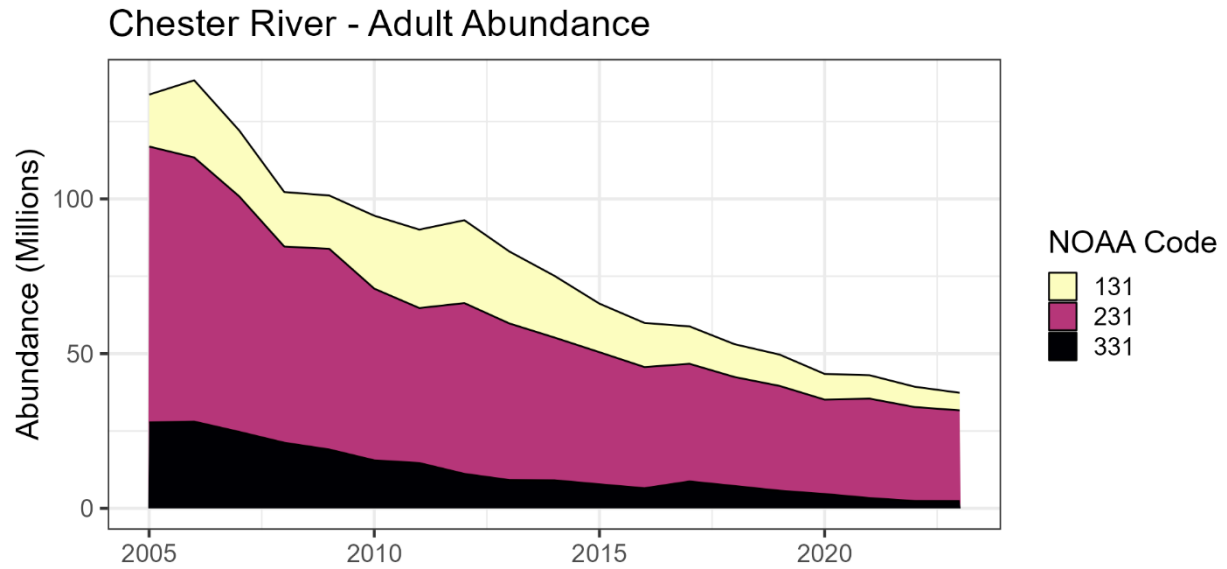
Figure 174. Estimated adult oyster abundance among modeled NOAA codes in the Chester River Region under Maryland management during 2005-2023.
