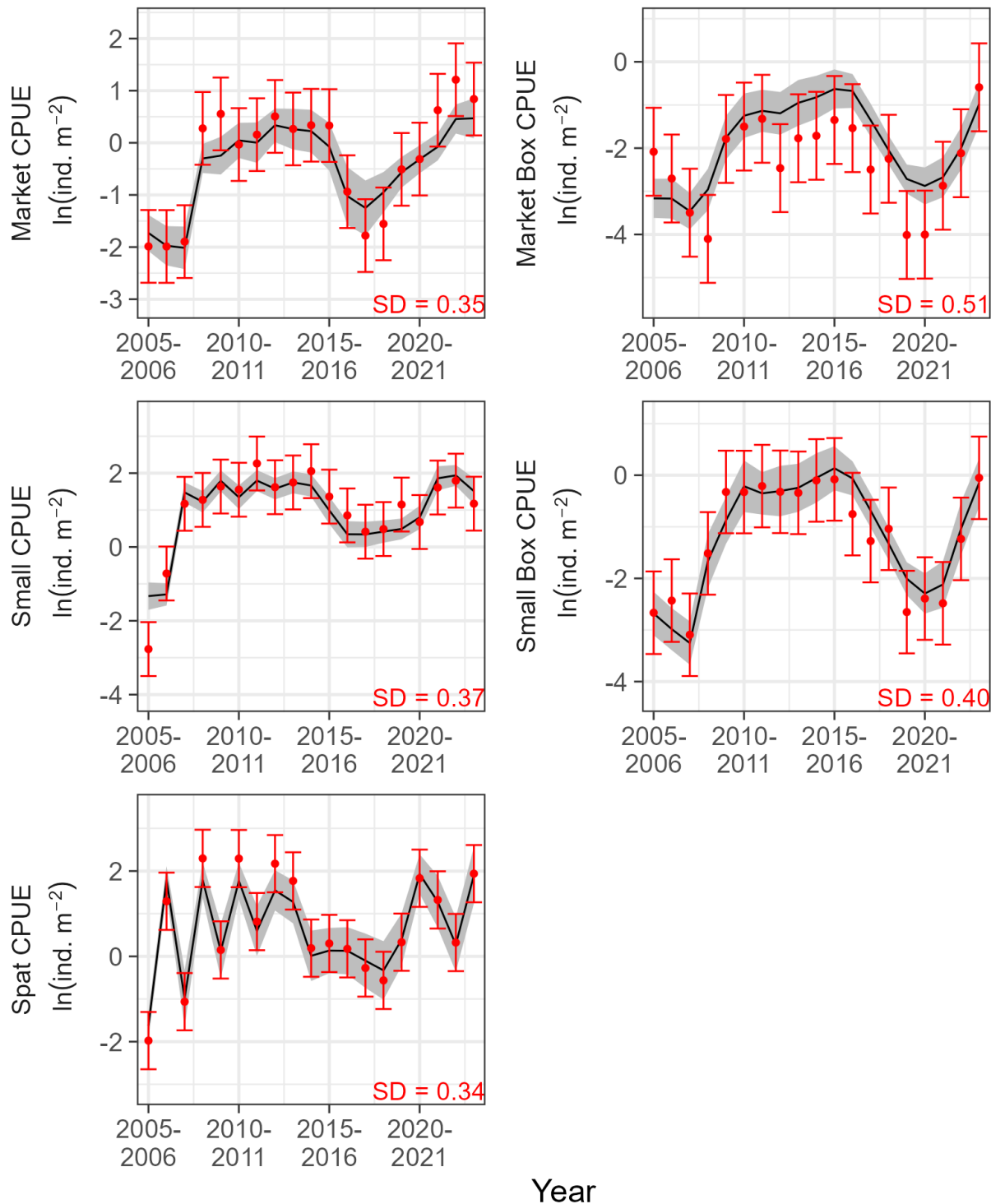
Figure 16. Estimated (line) and observed (points) values for Honga River. Variable and symbol definitions are the same as Figure 12.
