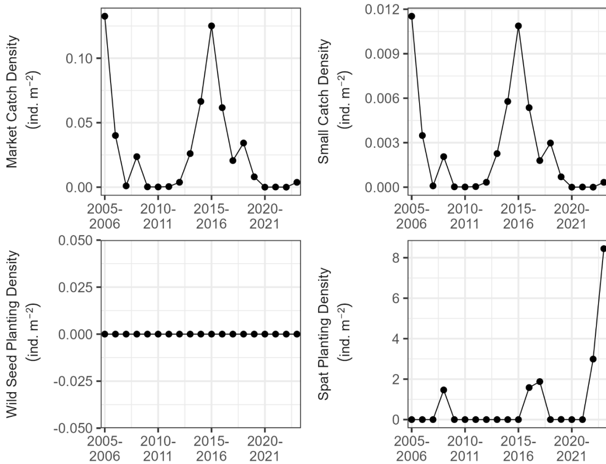
Figure 131. Catch density of market oysters, catch density of small oysters, wild seed planting density, and spat planting density during 2005-2023 in Miles River. Density was calculated as the number of individuals divided by habitat area for each data source.
