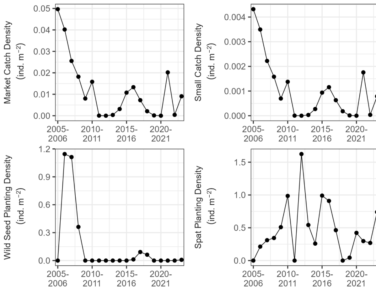
Figure 157. Catch density of market oysters, catch density of small oysters, wild seed planting density, and spat planting density during 2005-2023 in Upper Bay. Density was calculated as the number of individuals divided by habitat area for each data source.
