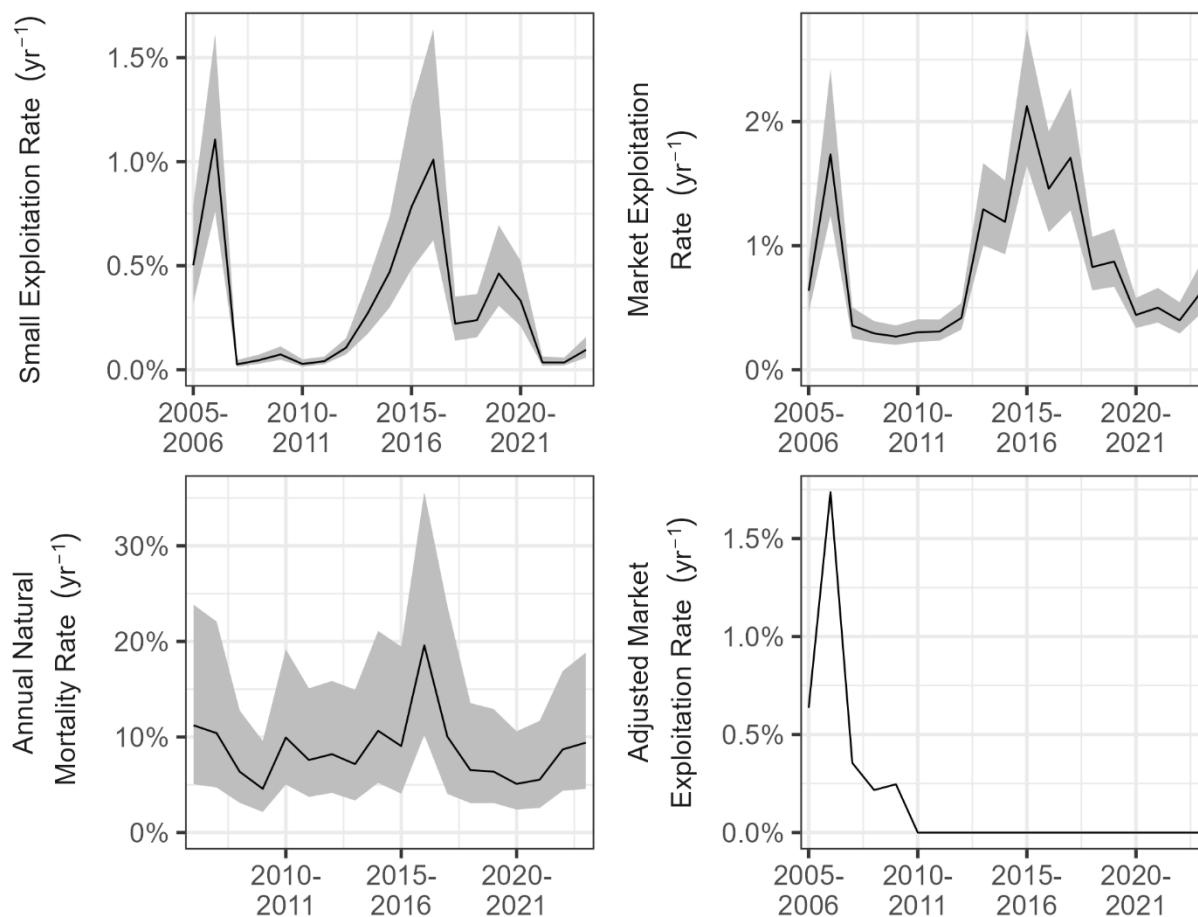
Figure 95. Estimated small exploitation rate, market exploitation rate, annual natural mortality rate, and adjusted market exploitation rate during 2005-2023 in Mid Choptank River. The shaded areas indicate approximate 95% confidence intervals.
