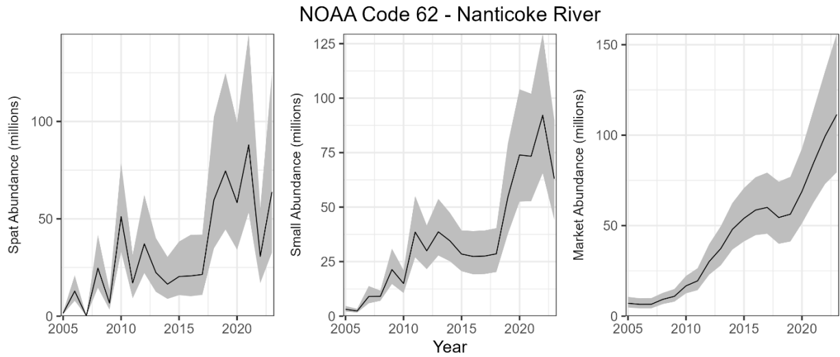
Figure 69. Estimated abundance of spat, small, and markets oysters during 2005-2023 in Nanticoke River. The lines indicate the estimated abundances, and the shaded areas indicate approximate 95% confidence intervals.
