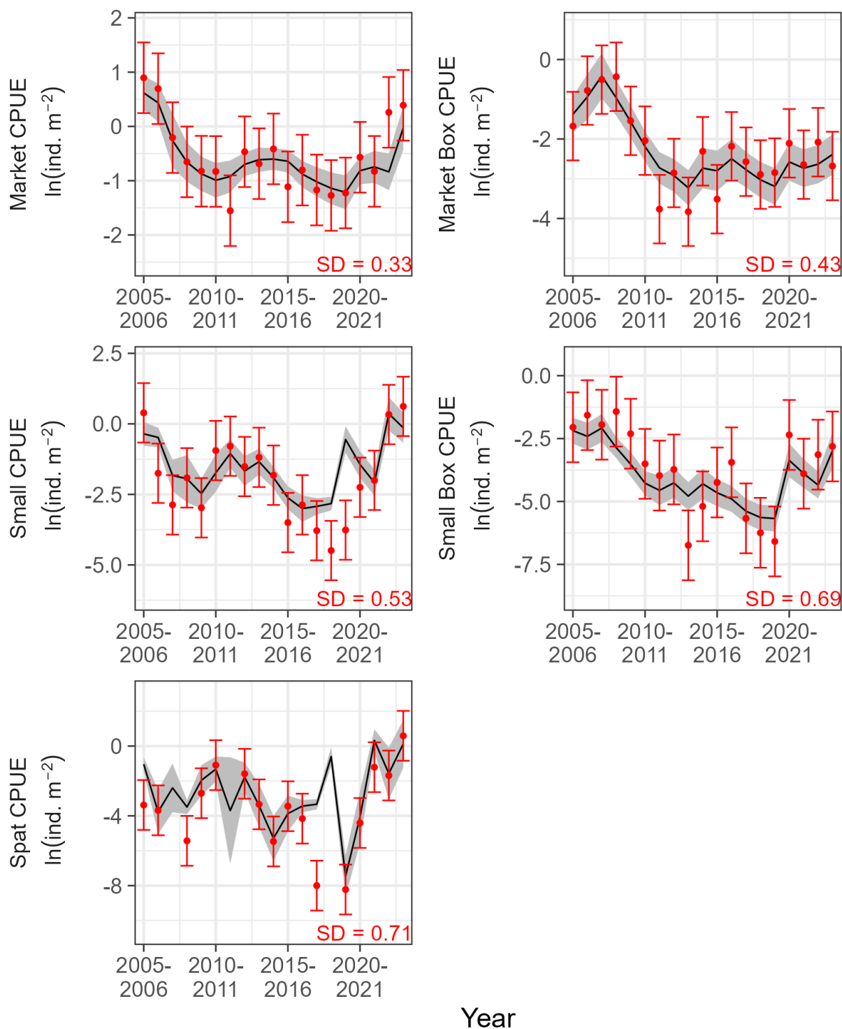
Figure 19. Estimated (line) and observed (points) values for the Miles River (NOAA code 60). Variable and symbol definitions are the same as Figure 12.
