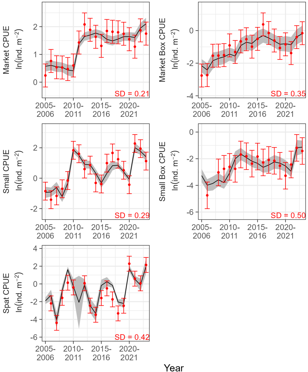
Figure 46. Estimated (line) and observed (points) values for Tred Avon River. Variable and symbol definitions are the same as Figure 12.
