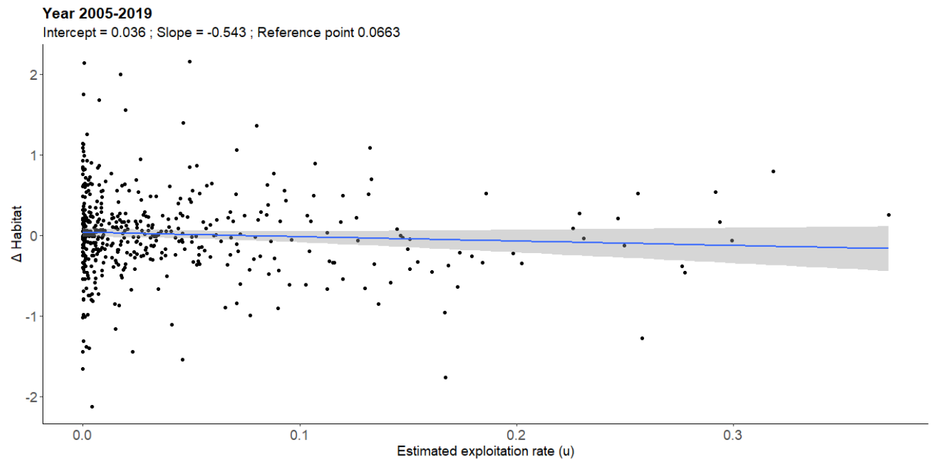
Figure 211 Results of sensitivity analysis for the exploitation rate reference point when using alternative ranges of years 2005-2019.
