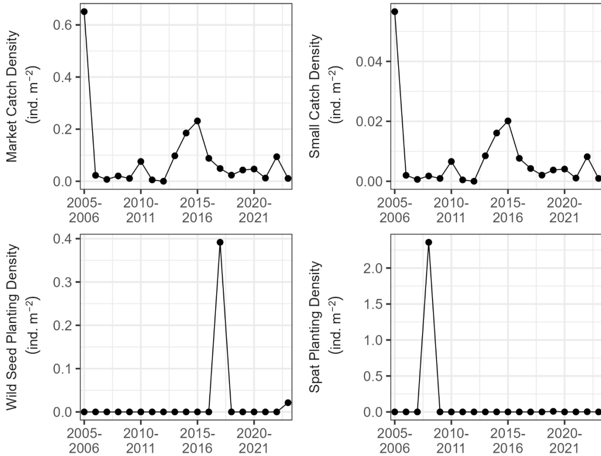
Figure 118. Catch density of market oysters, catch density of small oysters, wild seed planting density, and spat planting density during 2005-2023 in Mid Patuxent River. Density was calculated as the number of individuals divided by habitat area for each data source.
