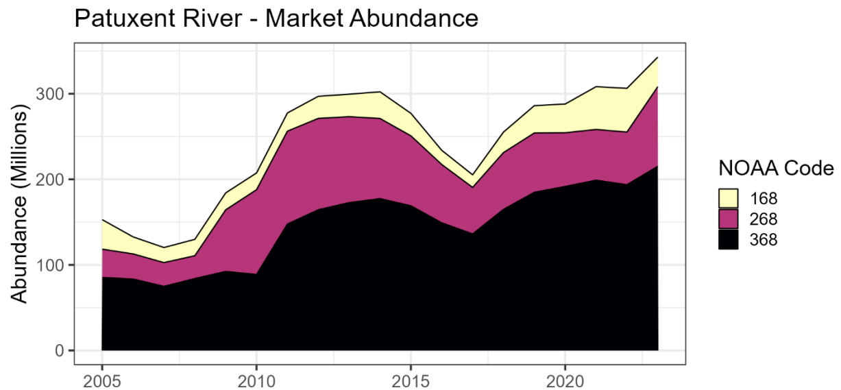
Figure 110. Estimated market oyster abundance among modeled NOAA codes in the Patuxent River Region under Maryland management during 2005-2023.
