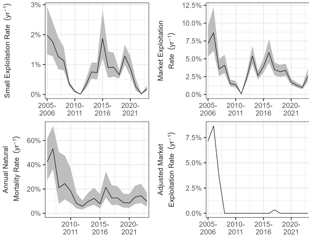
Figure 127. Estimated small exploitation rate, market exploitation rate, annual natural mortality rate, and adjusted market exploitation rate during 2005-2023 in Eastern Bay. The shaded areas indicate approximate 95% confidence intervals.
