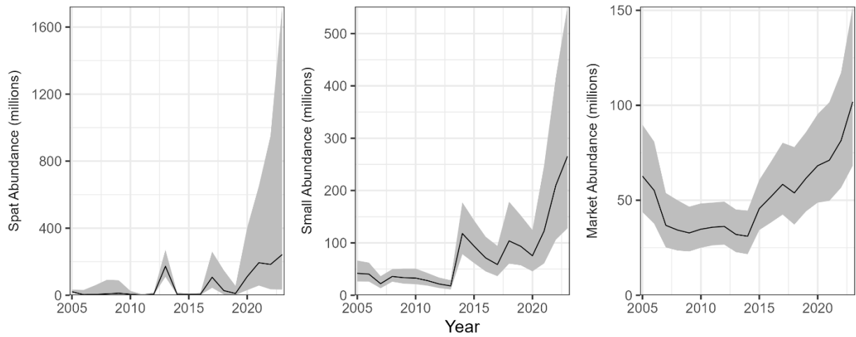
Figure 148. Estimated abundance of spat, small, and markets oysters during 2005-2023 in Wicomico River (West). The lines indicate the estimated abundances, and the shaded areas indicate approximate 95% confidence intervals.
