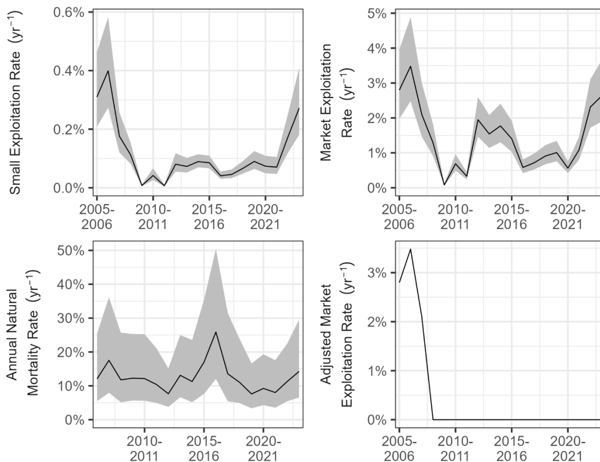
Figure 101. Estimated small exploitation rate, market exploitation rate, annual natural mortality rate, and adjusted market exploitation rate during 2005-2023 in Harris Creek. The shaded areas indicate approximate 95% confidence intervals.
