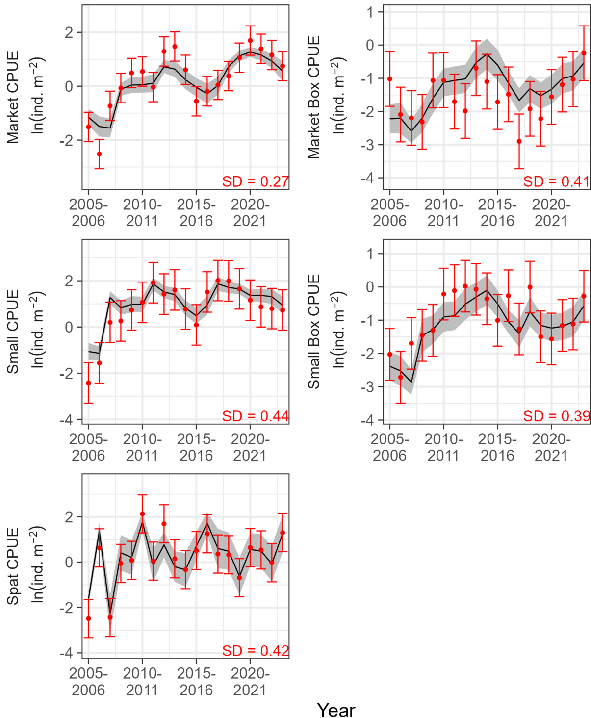
Figure 40. Estimated (line) and observed (points) values for Tangier Sound North. Variable and symbol definitions are the same as Figure 12.
