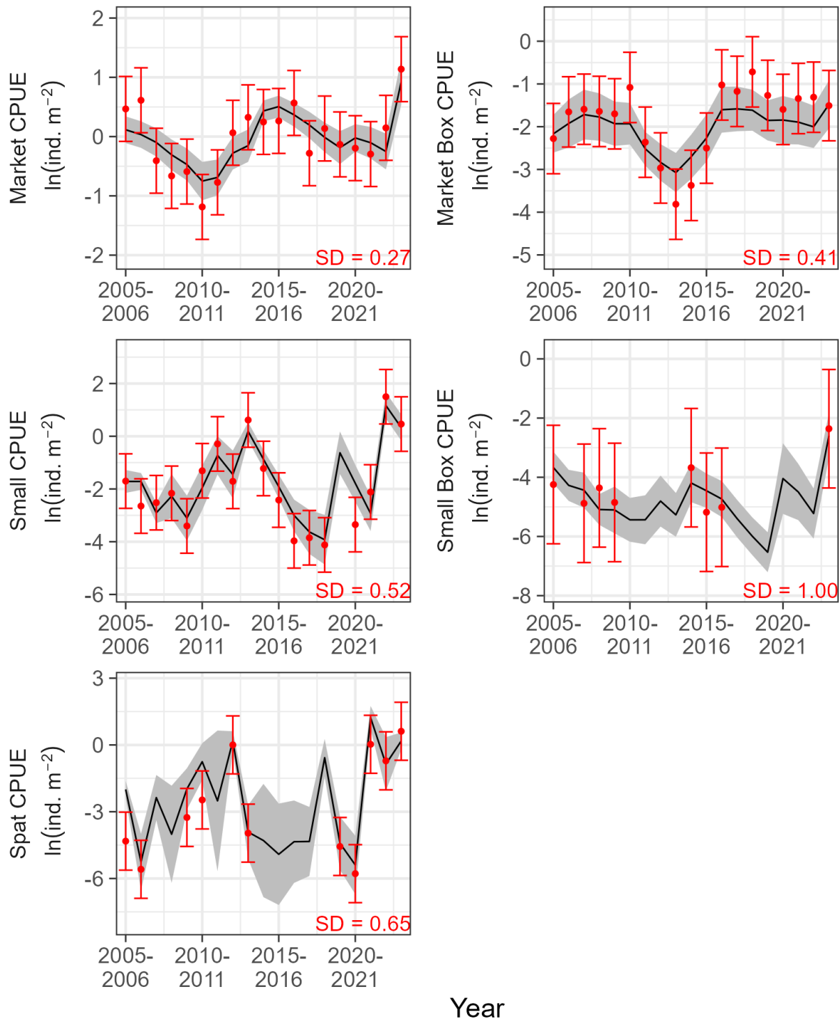
Figure 27. Estimated (line) and observed (points) values for Wye River. Variable and symbol definitions are the same as Figure 12.
