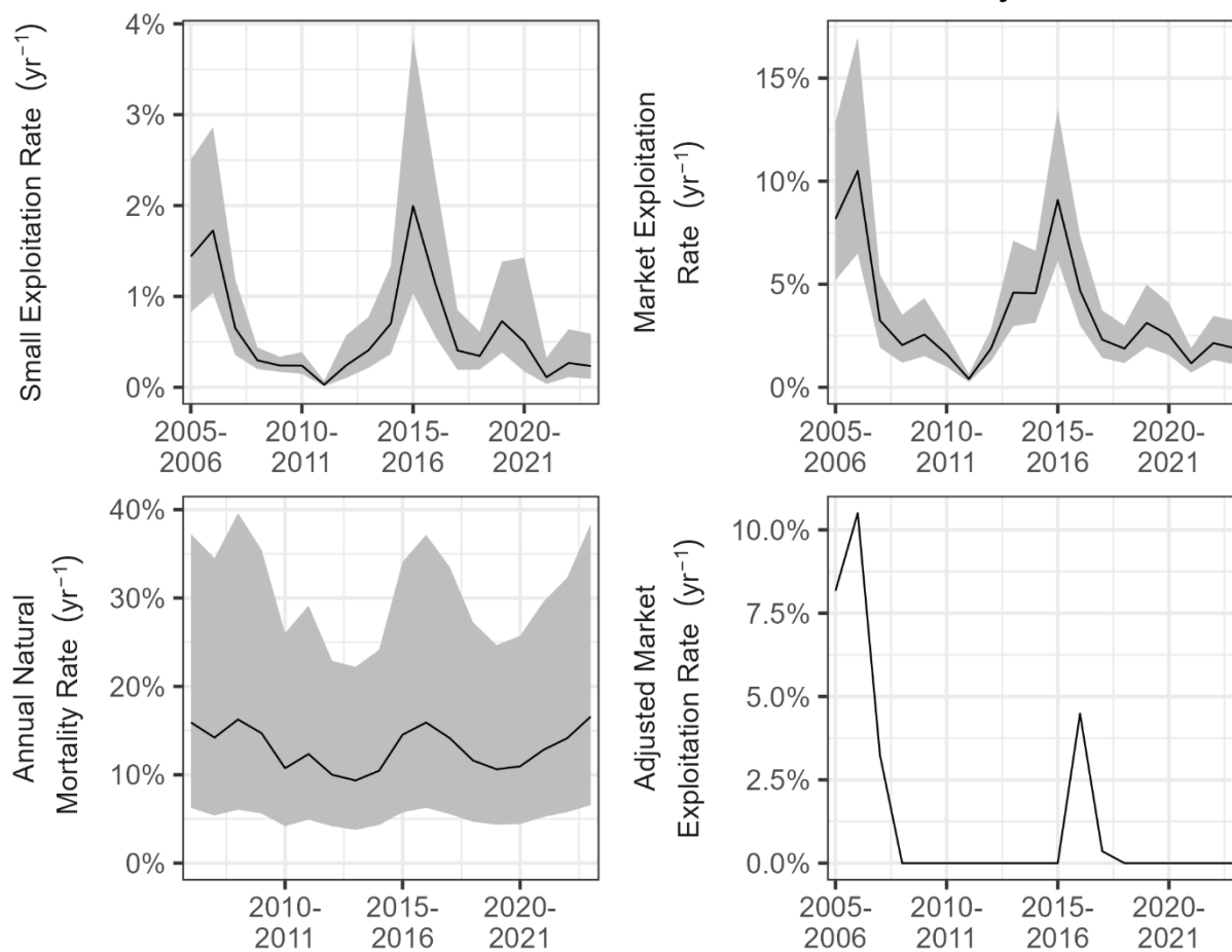
Figure 159. Estimated small exploitation rate, market exploitation rate, annual natural mortality rate, and adjusted market exploitation rate during 2005-2023 in South Mid-Bay. The shaded areas indicate approximate 95% confidence intervals.
