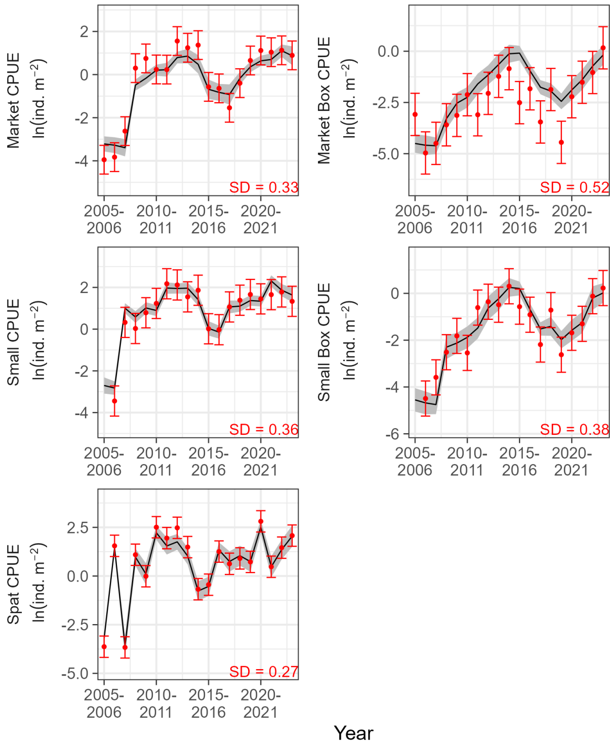
Figure 15. Estimated (line) and observed (points) values for Fishing Bay. Variable and symbol definitions are the same as Figure 12.
