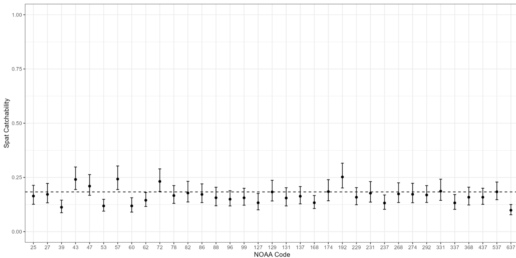
Figure 49. Estimated spat catchability for the Fall Dredge Survey in each NOAA code (points) with approximate 95% confidence intervals (whiskers). The dashed line represents the median of the penalty included in the model.
