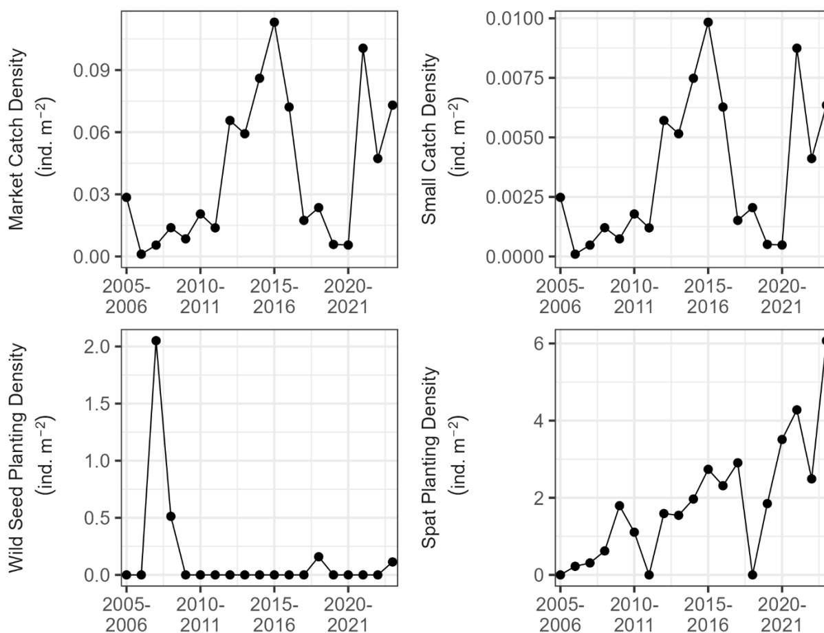
Figure 150. Catch density of market oysters, catch density of small oysters, wild seed planting density, and spat planting density during 2005-2023 in Wicomico River (West). Density was calculated as the number of individuals divided by habitat area for each data source.
