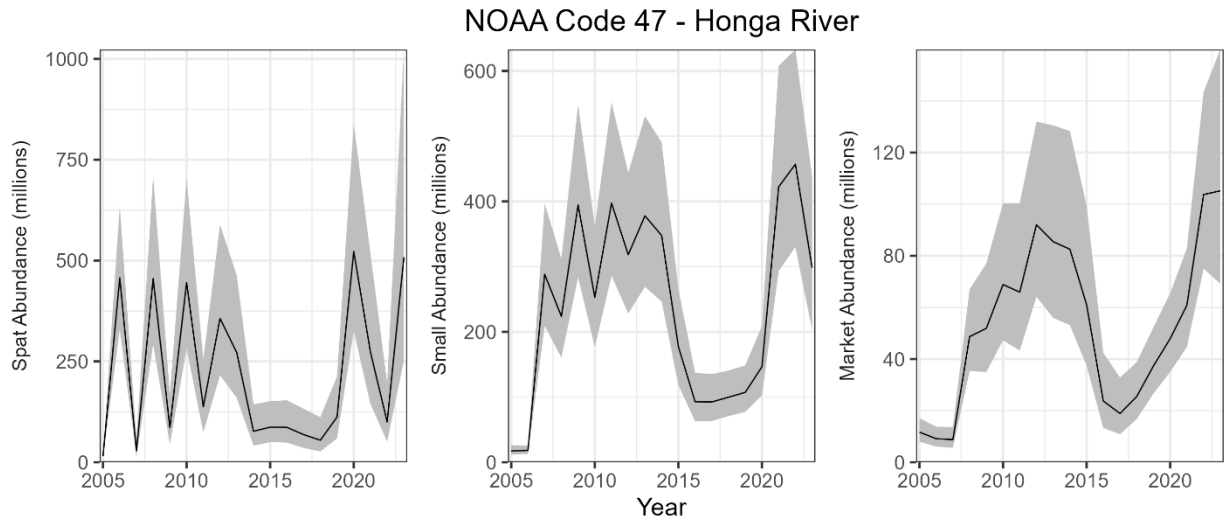
Figure 63. Estimated abundance of spat, small, and markets oysters during 2005-2023 in Honga River. The lines indicate the estimated abundances, and the shaded areas indicate approximate 95% confidence intervals.
