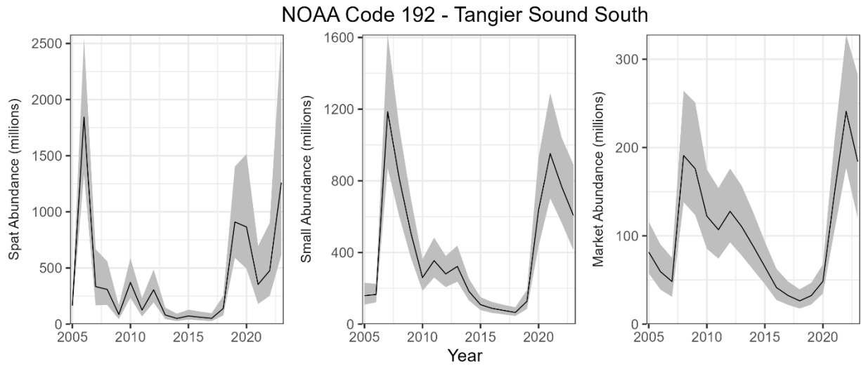
Figure 78. Estimated abundance of spat, small, and markets oysters during 2005-2023 in Tangier Sound South. The lines indicate the estimated abundances, and the shaded areas indicate approximate 95% confidence intervals.
