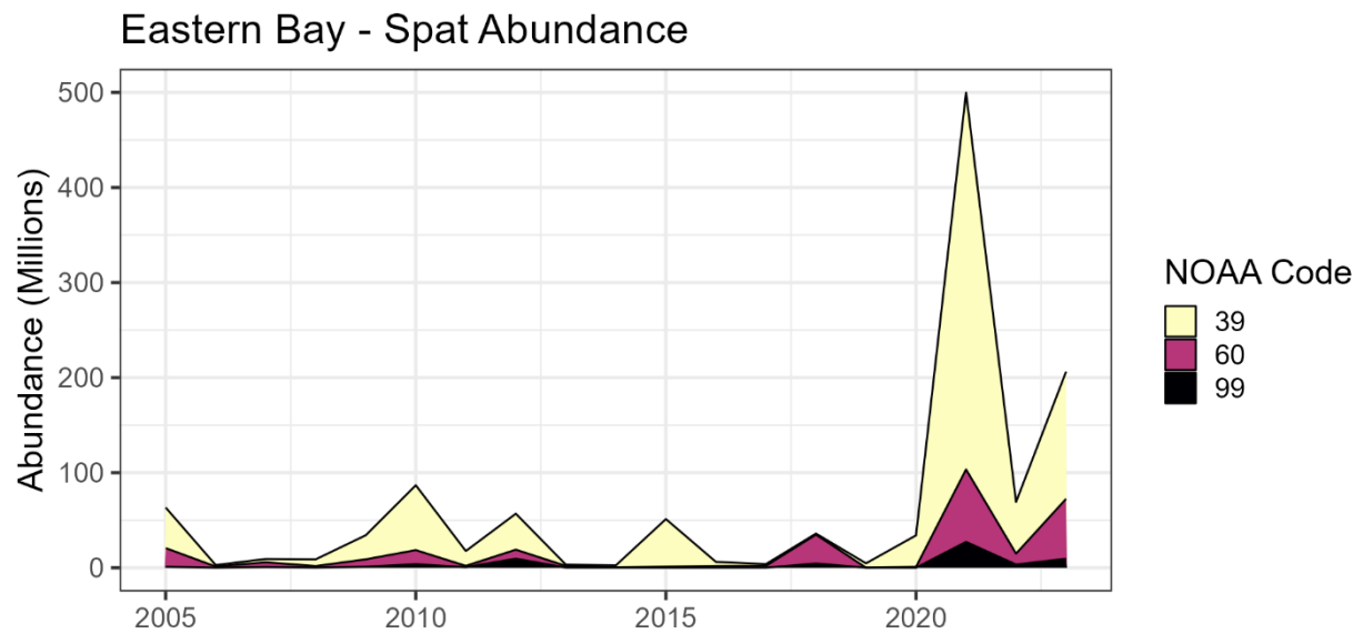
Figure 125. Estimated spat oyster abundance among modeled NOAA codes in the Eastern Bay Region under Maryland management during 2005-2023.
