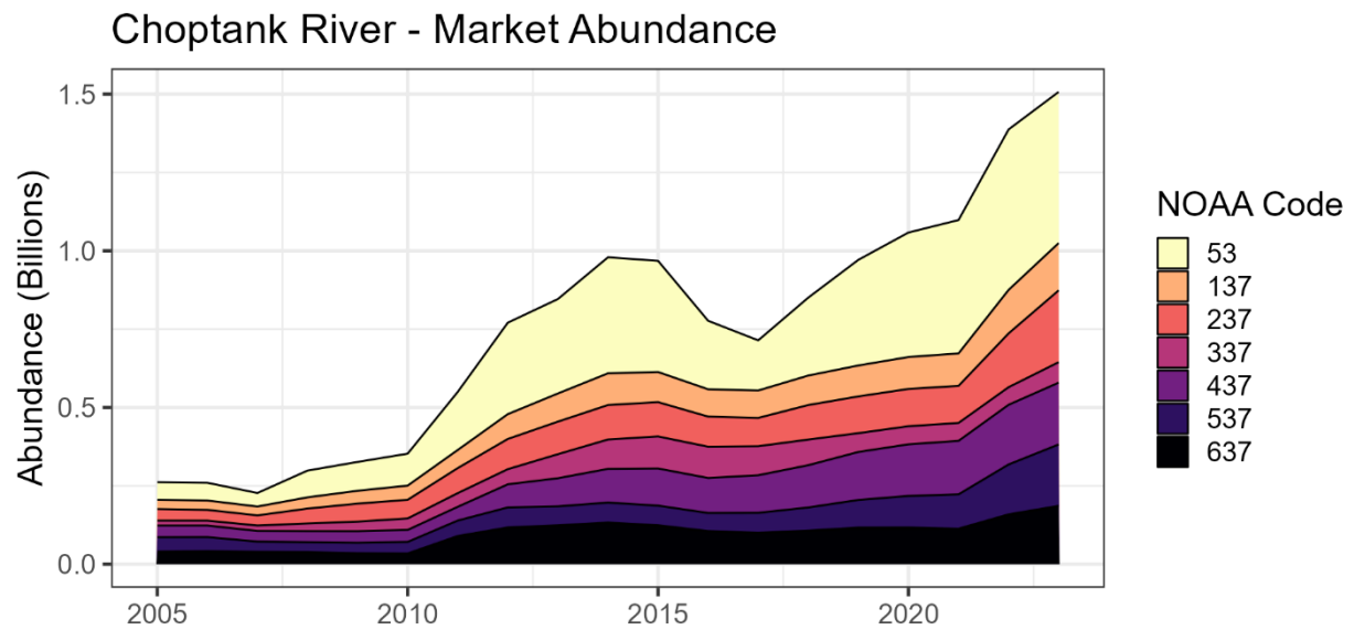
Figure 85. Estimated market oyster abundance among modeled NOAA codes in the Choptank River Region under Maryland management during 2005-2023.
