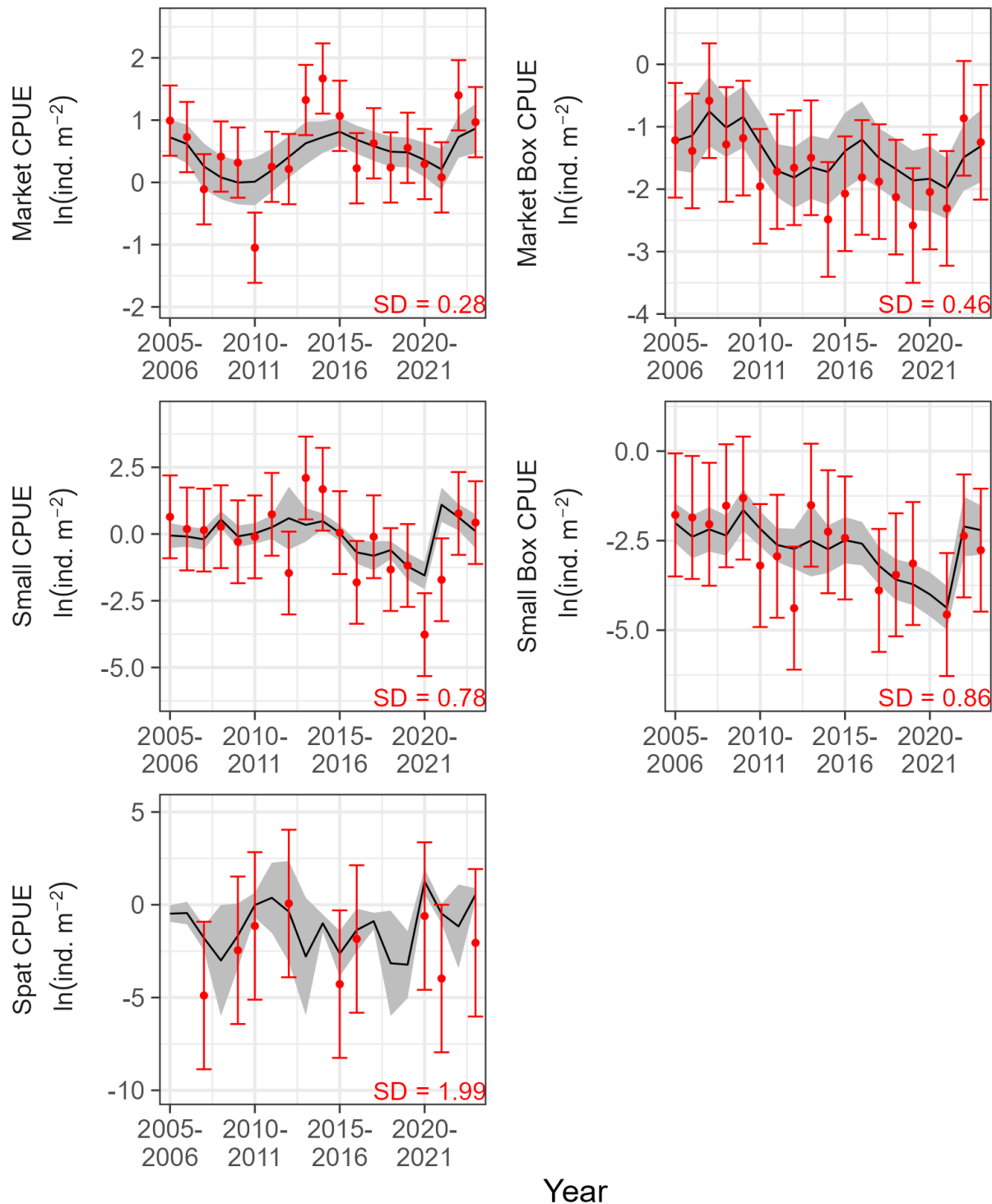
Figure 25. Estimated (line) and observed (points) values for South River. Variable and symbol definitions are the same as Figure 12.
